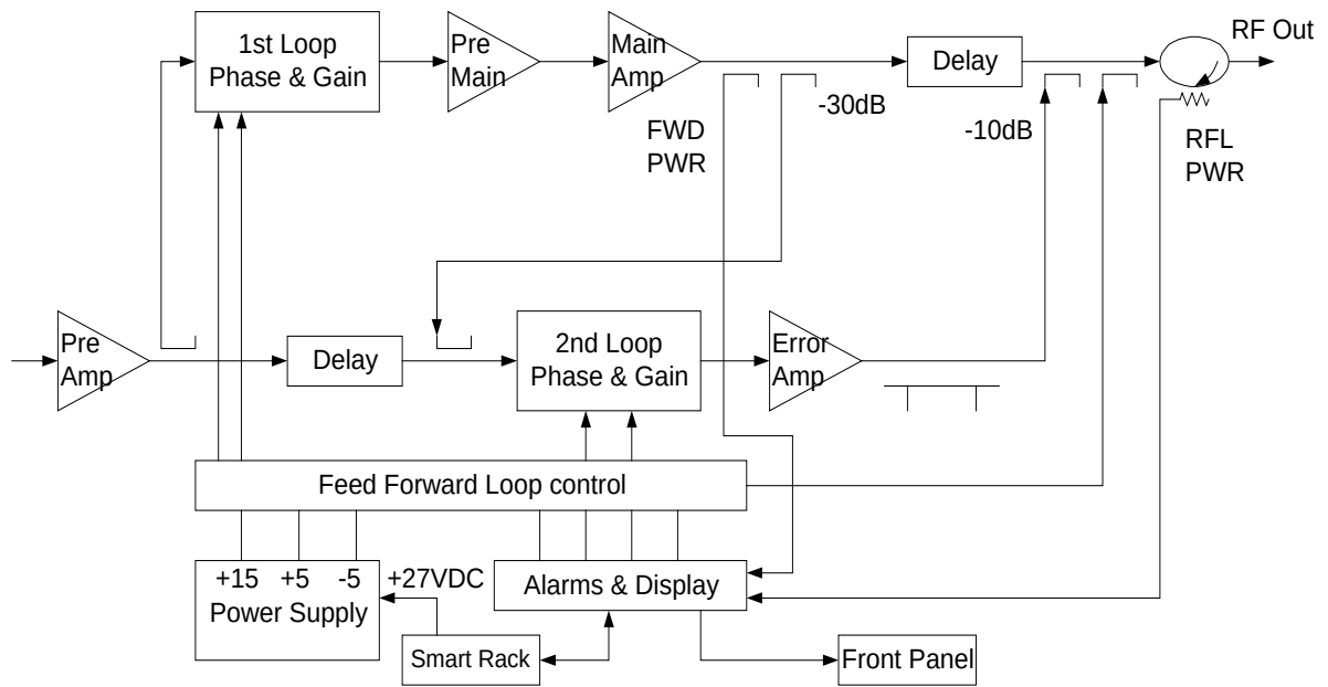
G3S-800-140 Functional Block Diagram
