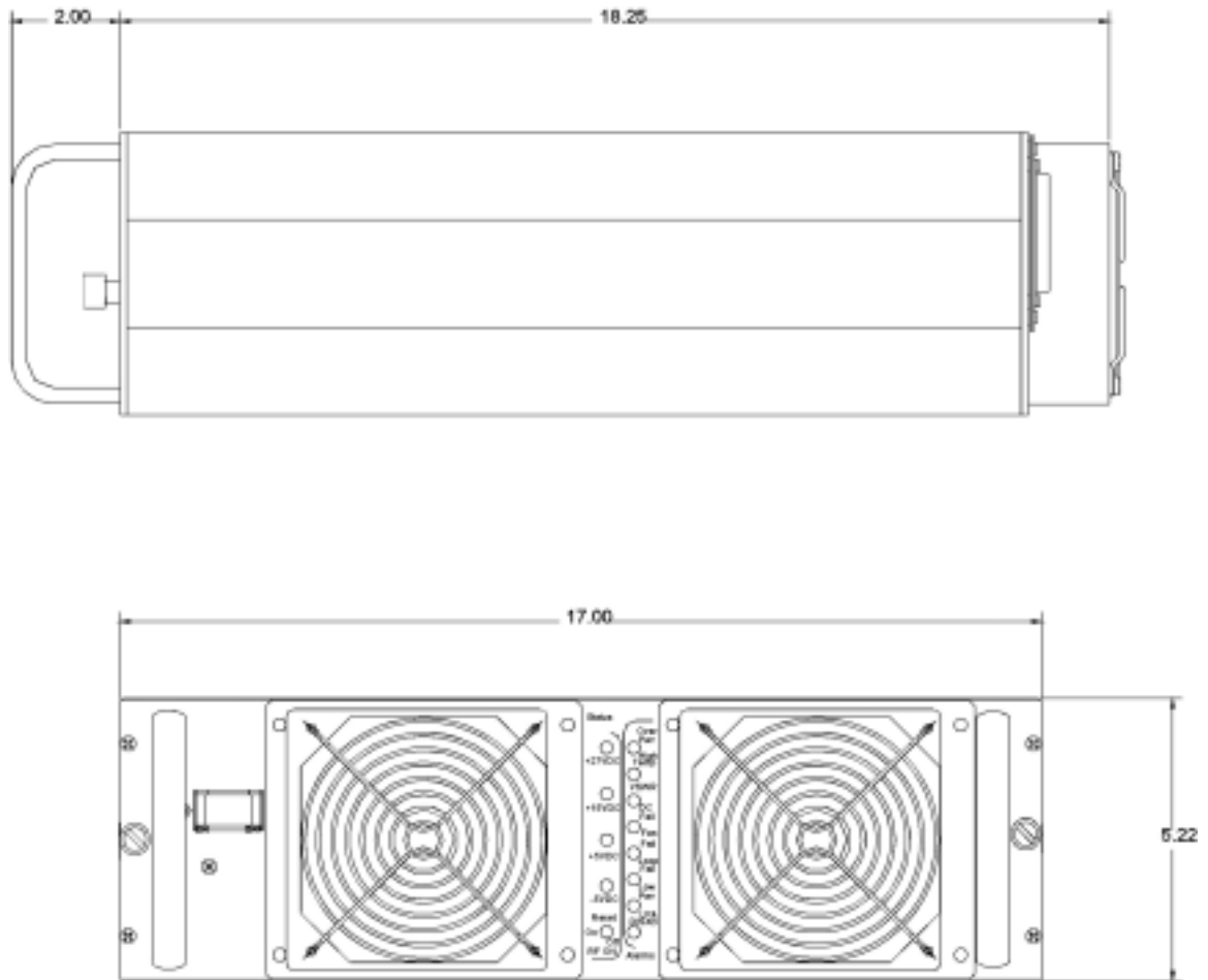
Figure 1-1 G3S-800-140
