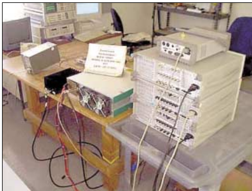
Direct Connect at Antenna Port Test Setup - Back
