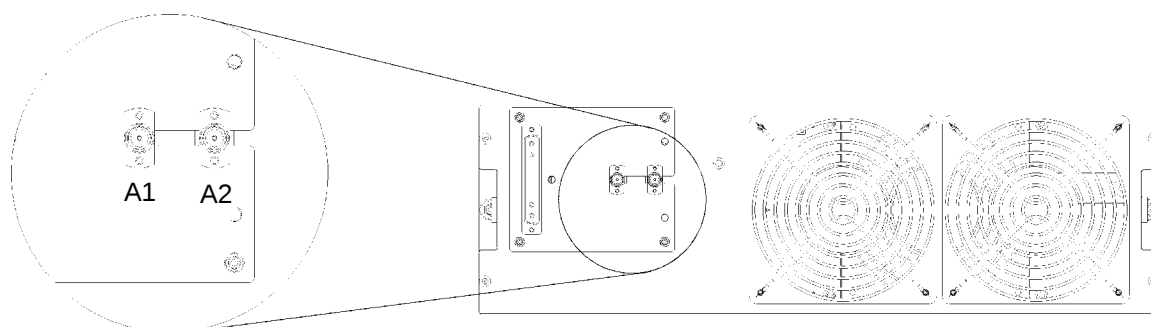
Figure 2-3 Amplifier RF Connector
