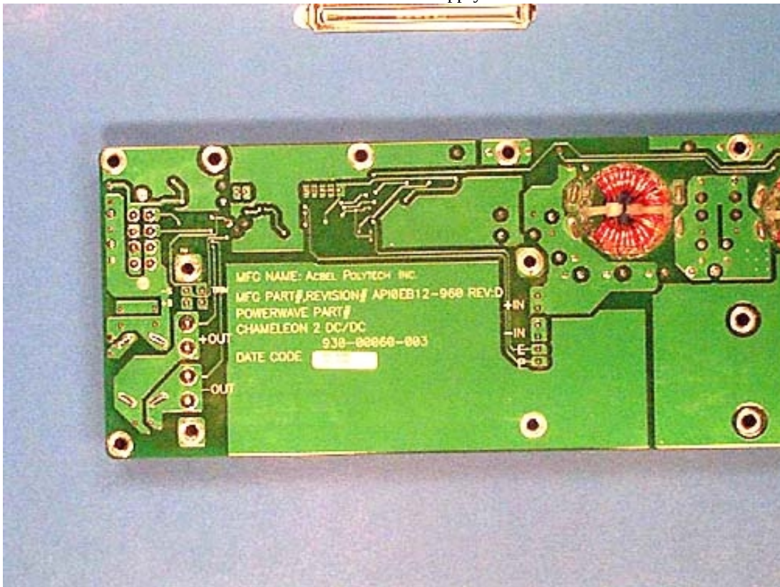
DC Power Supply
