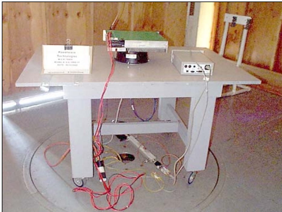
OATS Test Setup - Back View - AC
