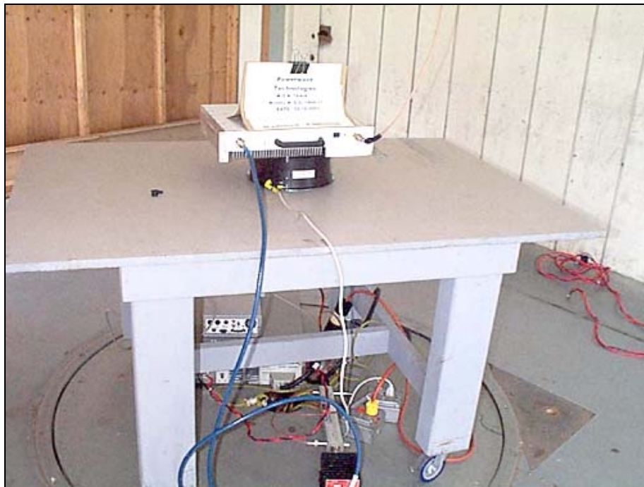
OATS Test Setup - Front View - DC
