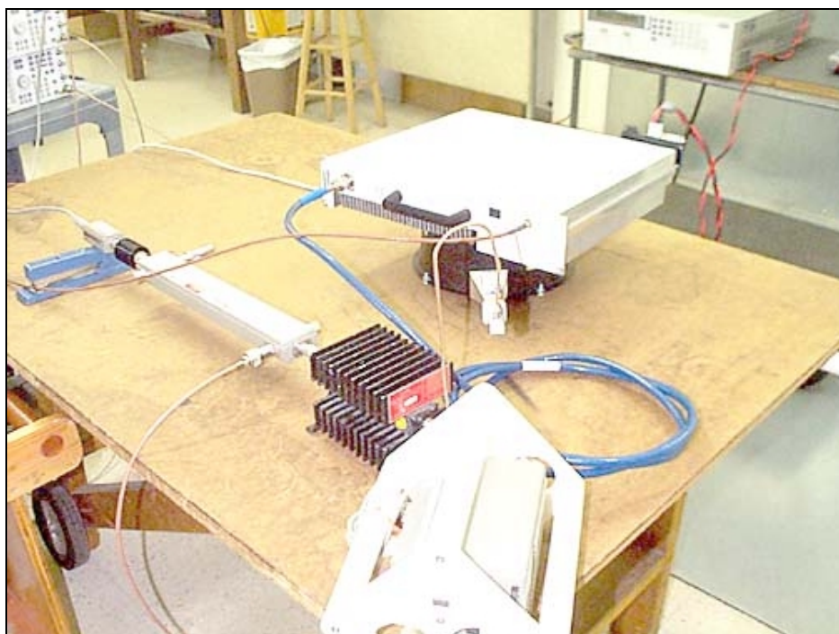
OATS Test Setup - Back View - DC 18-20 GHz
