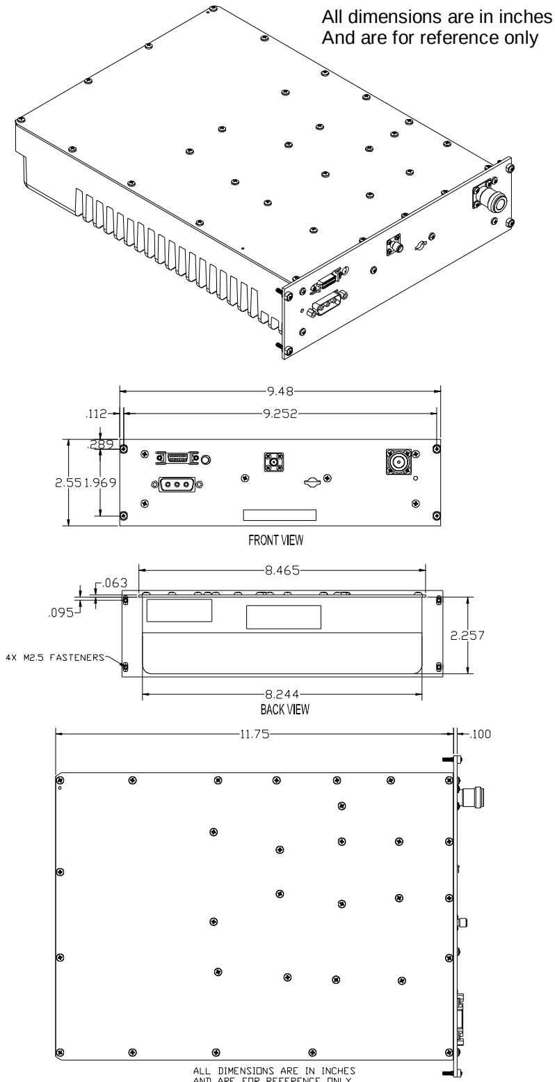
Figure 1-1. SPA 9321-30C Amplifier
