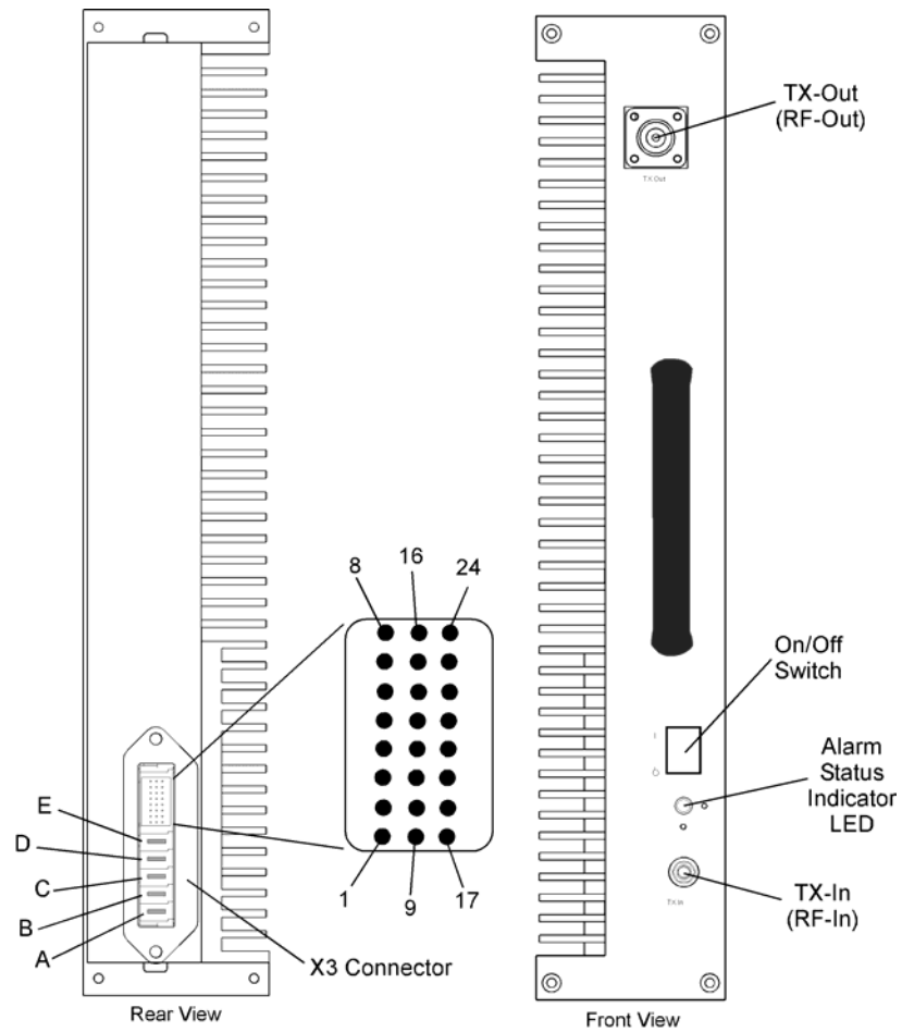
Figure 1-1 G3L-2100-30-B and G3L-2100-30-C Front and Rear Views
