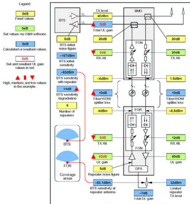
Figure 6-9. Nine FORs, high optical loss, high total uplink gain
