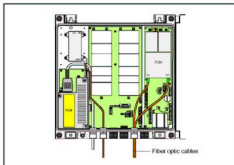
Figure 6-2. Fiber connection in a slave unit
