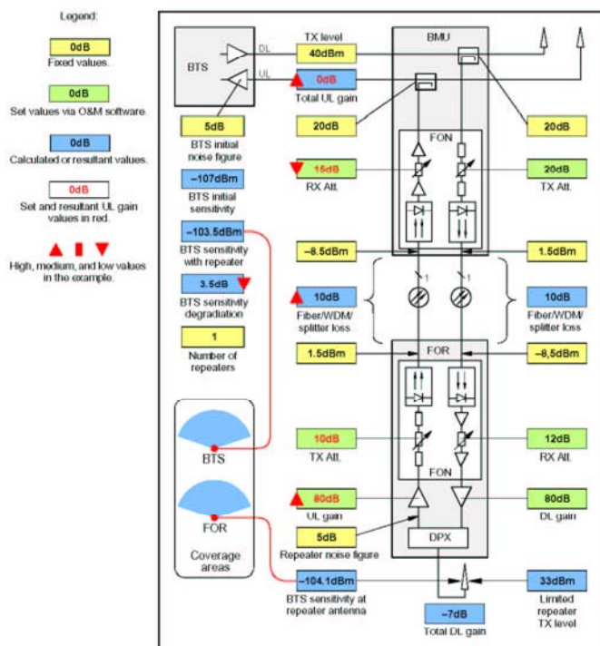
Figure 6-7. One FOR, high optical loss, high uplink gain
