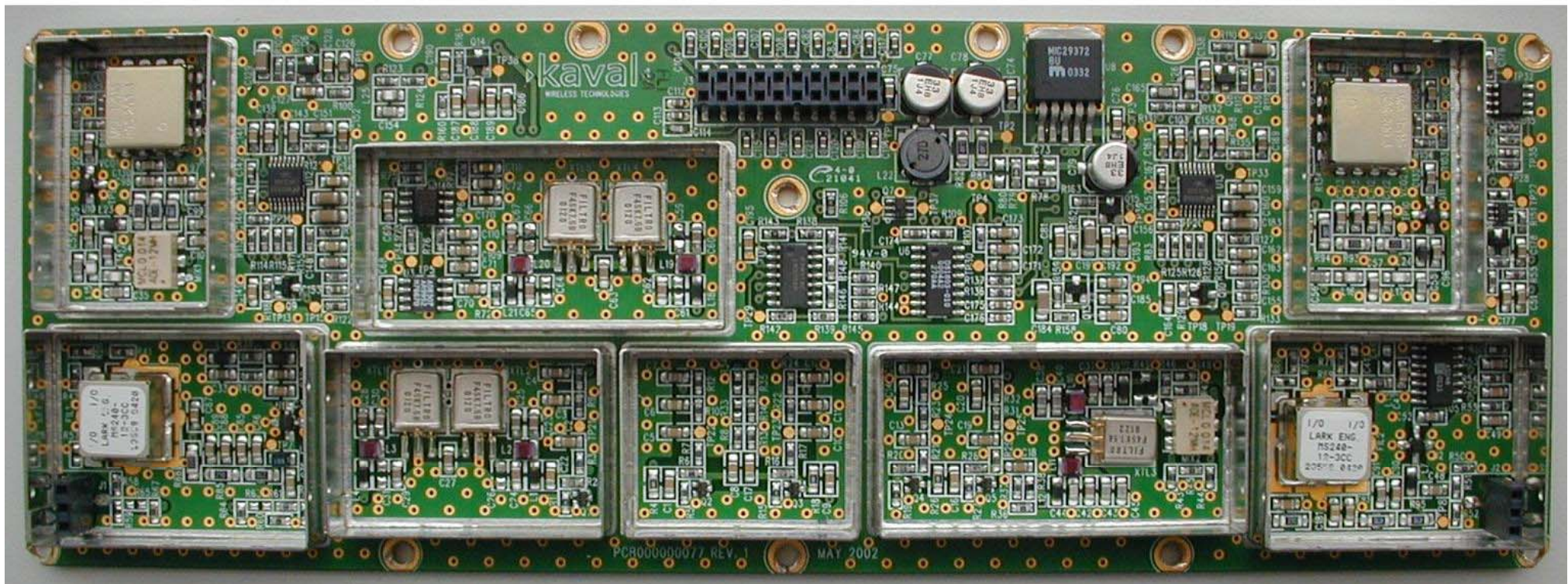
IF Board Top
