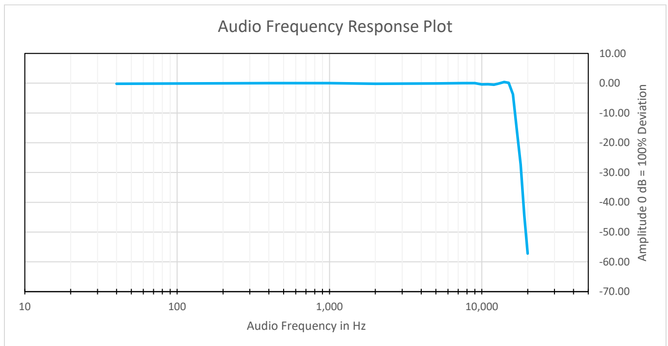
Figure 3—Equipment set-up audio frequency response (constant input)
