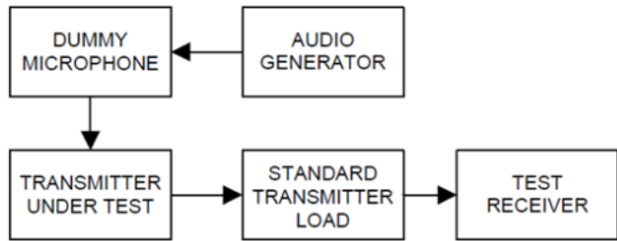
Figure 1—Equipment set-up for modulation limiting test
