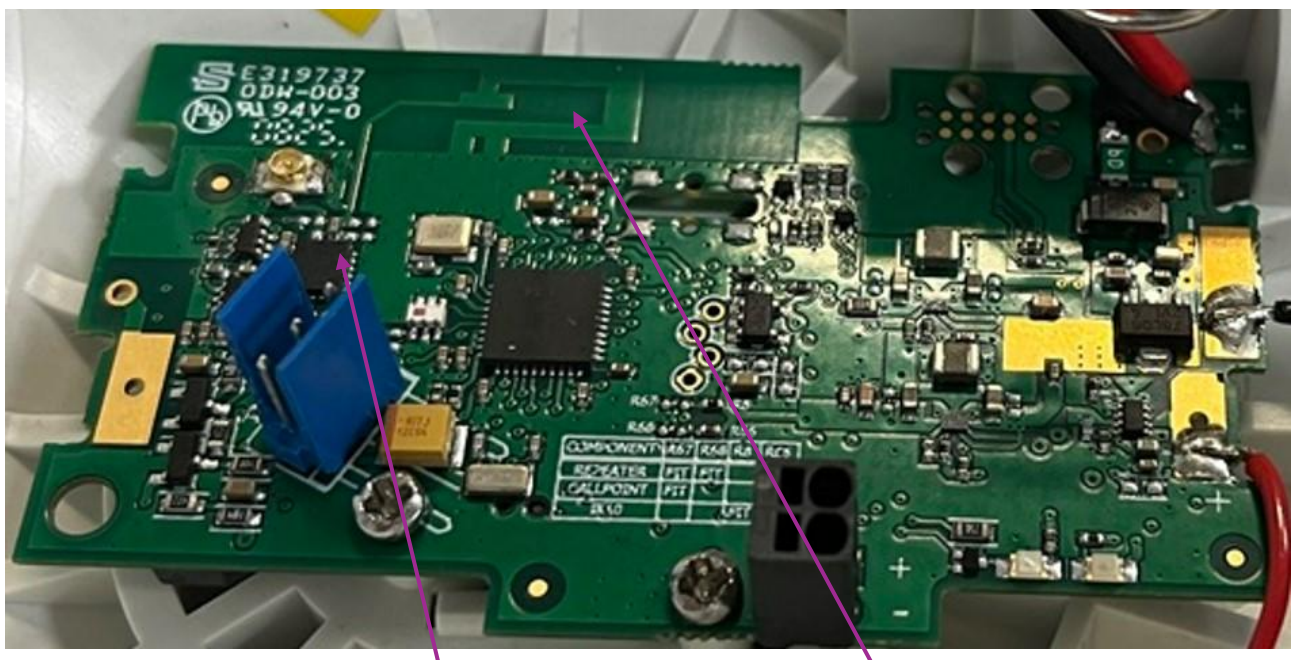
PCB Front
