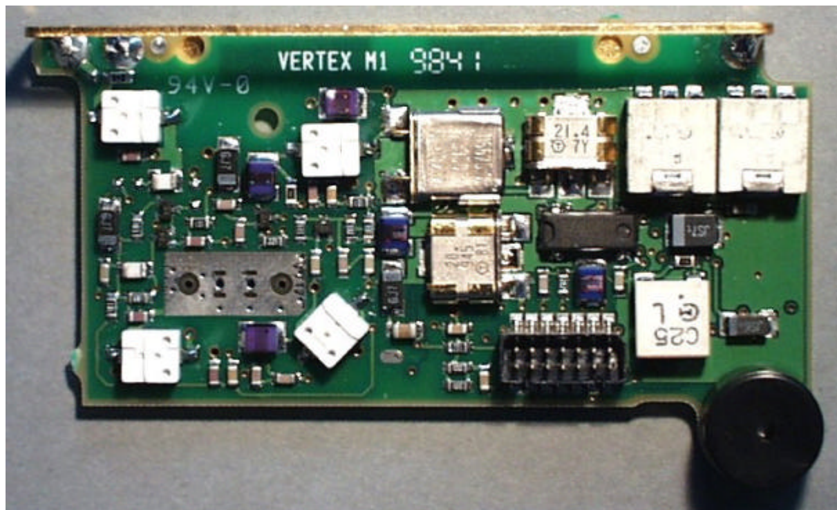
TLA852/FLA872 - RADIO PCB FRONT VIEW
