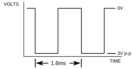
WAVEFORM AT PIN 39
