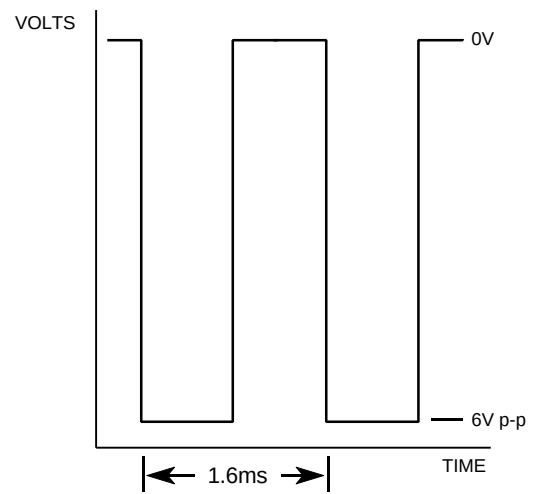
WAVEFORM AT PIN 41
