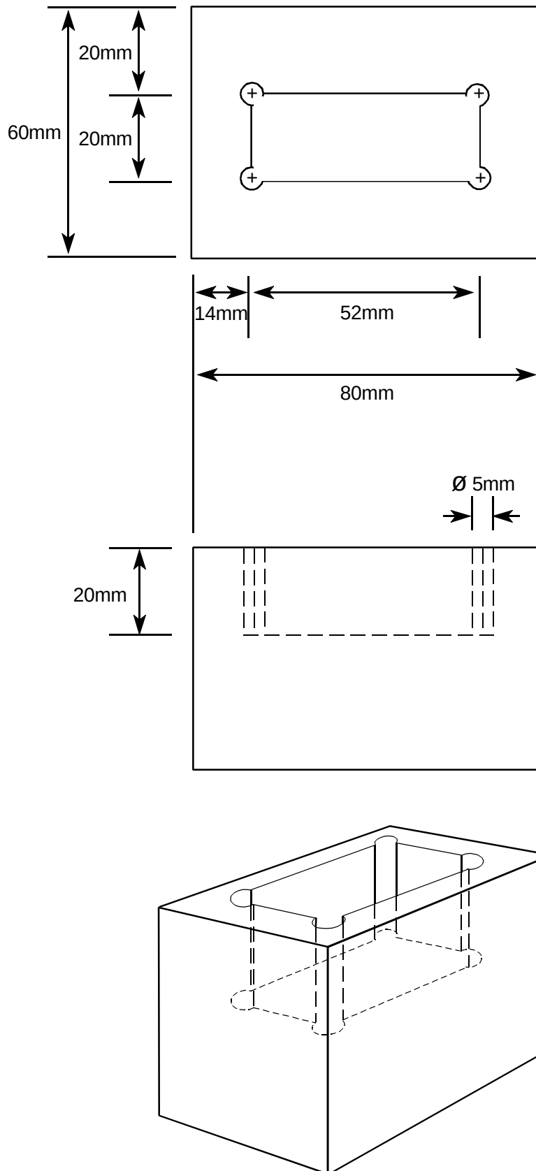
Figure 5.14: Polystyrene Block for TEM Cell Test - Dimensions
