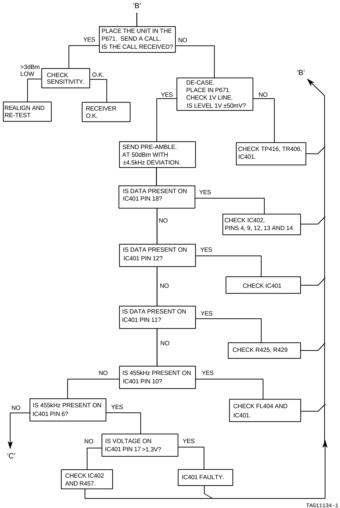
Figure 5.6: Fault Finding Guide (Sheet 2 of 3)
