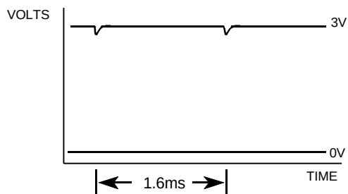
WAVEFORM AT PIN 45
