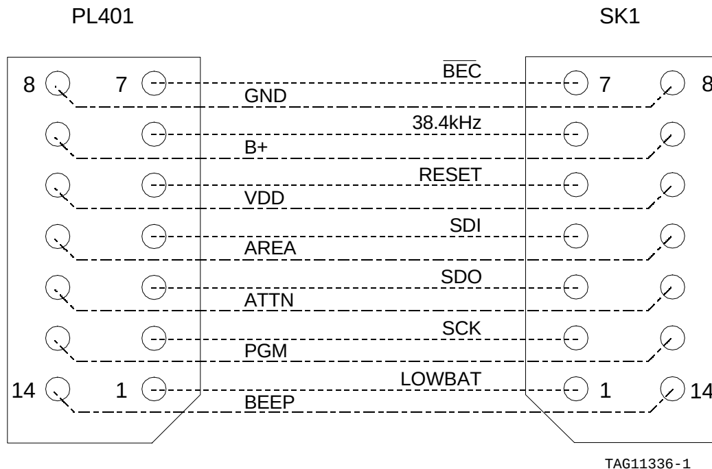
Figure 5.4: Connections between Radio Board and Decoder Board
