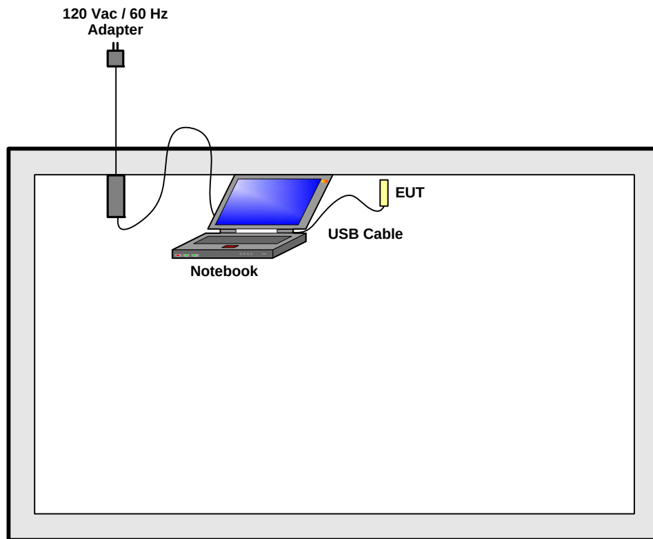
Test Setup Diagram - Radiated Emission (Above 1GHz)
