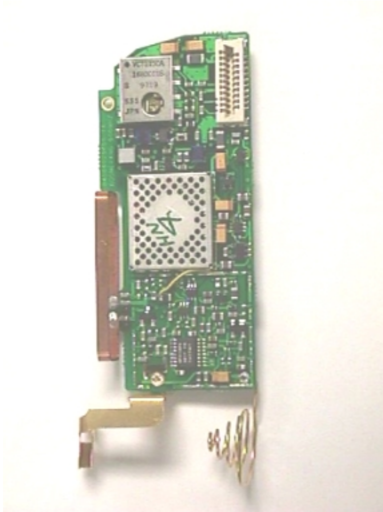
Transceiver Board Bottom View
