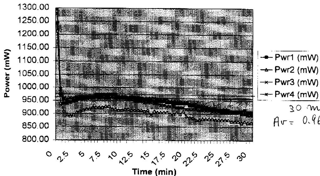
Boomerang Avg conducted TX power vs. time
