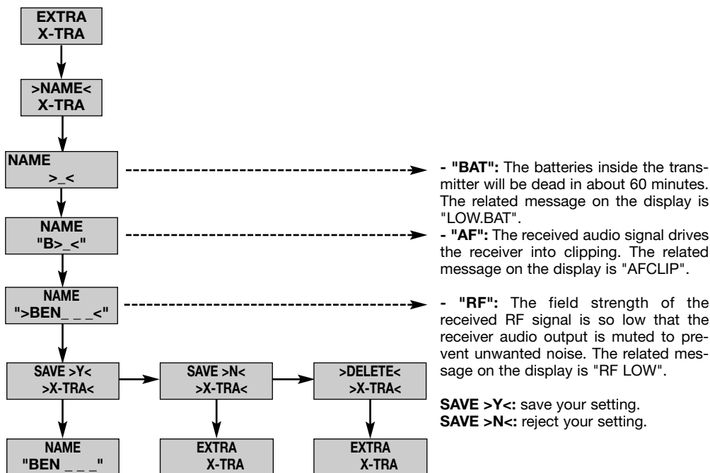
Diagram 13: Warning messages.
