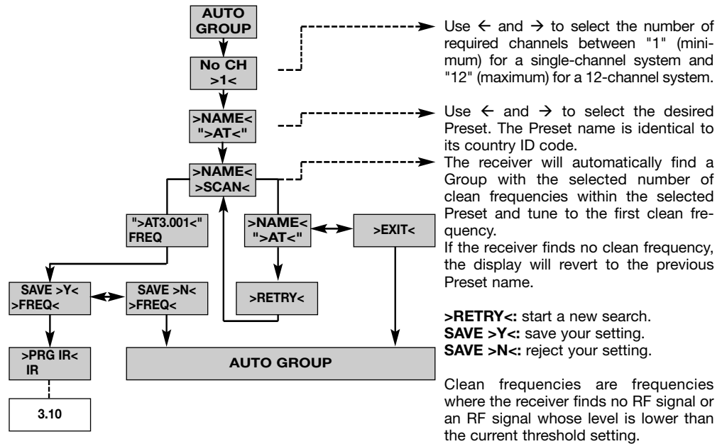
Diagram 3: Automatic search for a clean (interference-free) Frequency Group.
