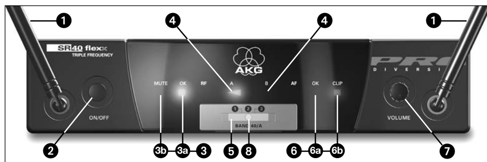
Fig. 1: Front panel controls on SR 40 FLEXX receiver.
