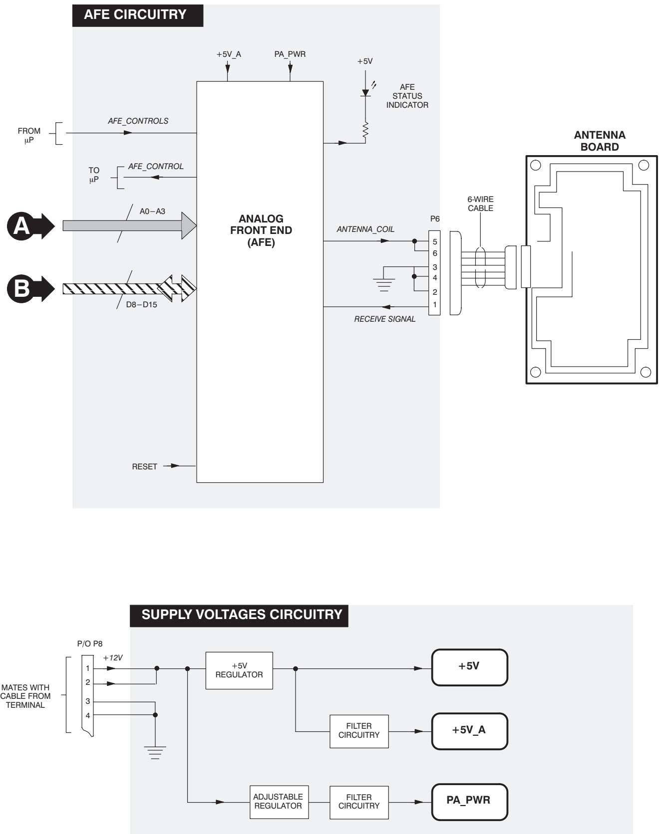
Figure 1. Card Access Device (CAD) Functional Block Diagram (2 of 2)
