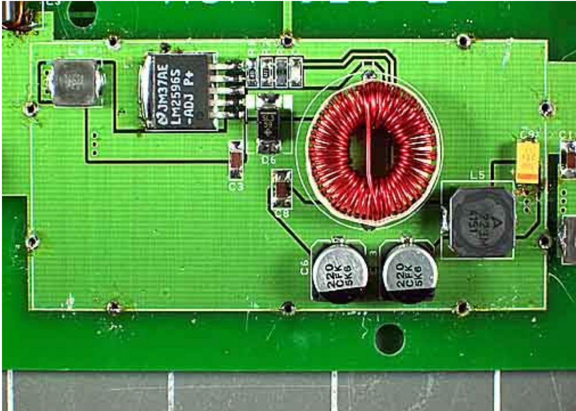
Main PCB Top Closeup Antenna Output with Shield Removed
