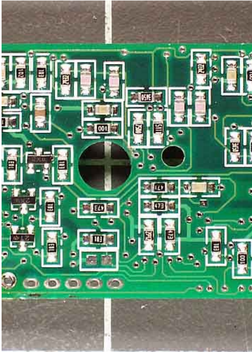
TX PCB Bottom Closeup 2
