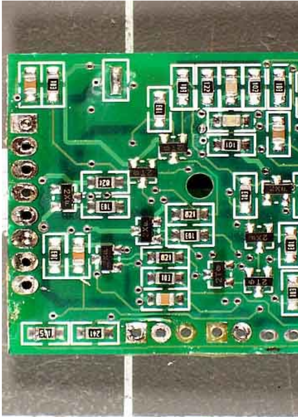
TX PCB Bottom Closeup 3
