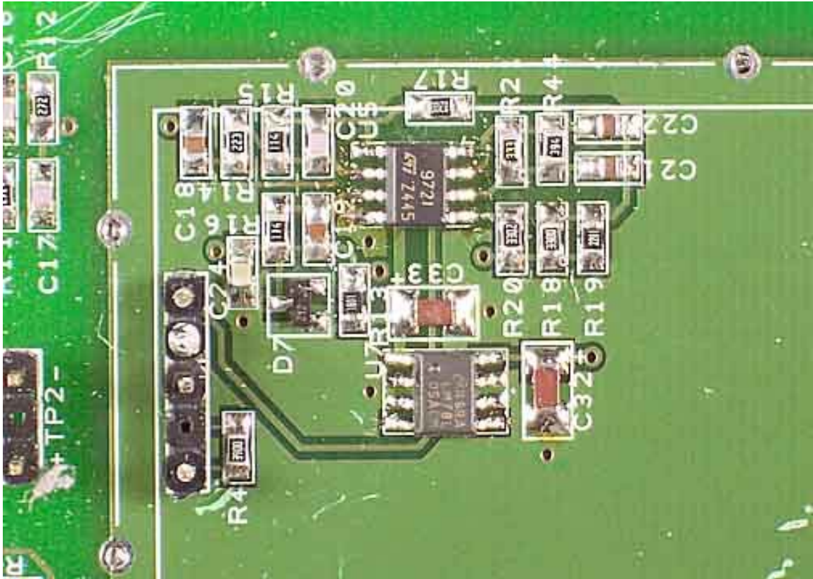
Main PCB Top Closeup TX Underside Closeup
