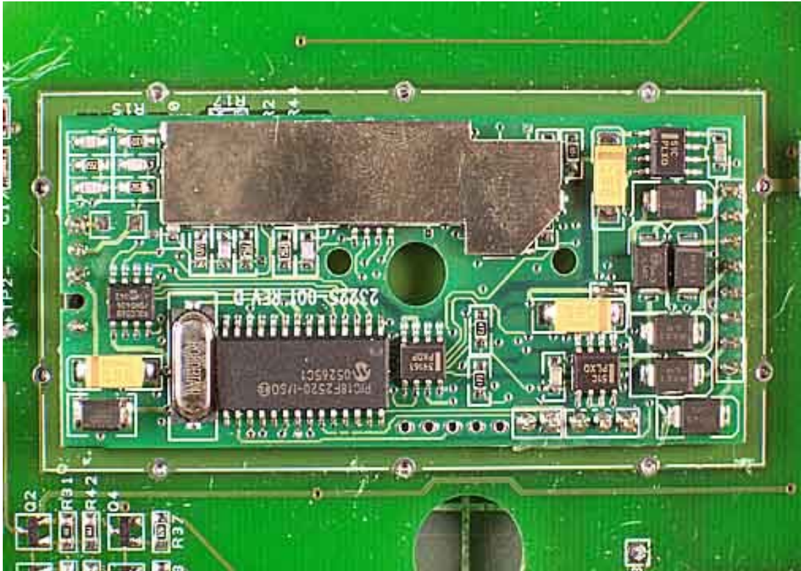
Main PCB Top Closeup TX Underside Closeup with Shield Removed
