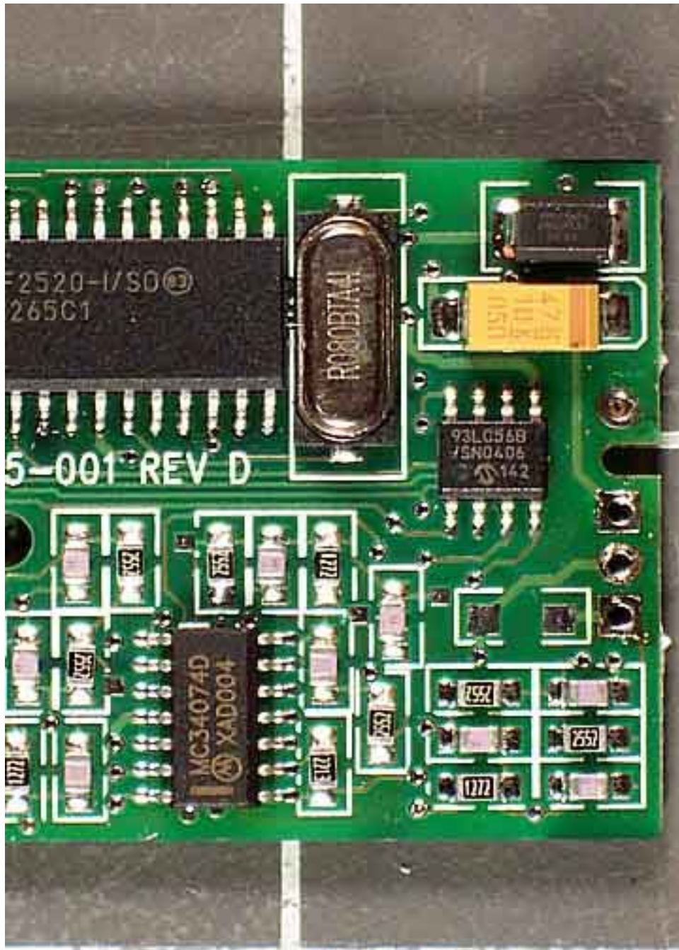
TX PCB Top Closeup 1
