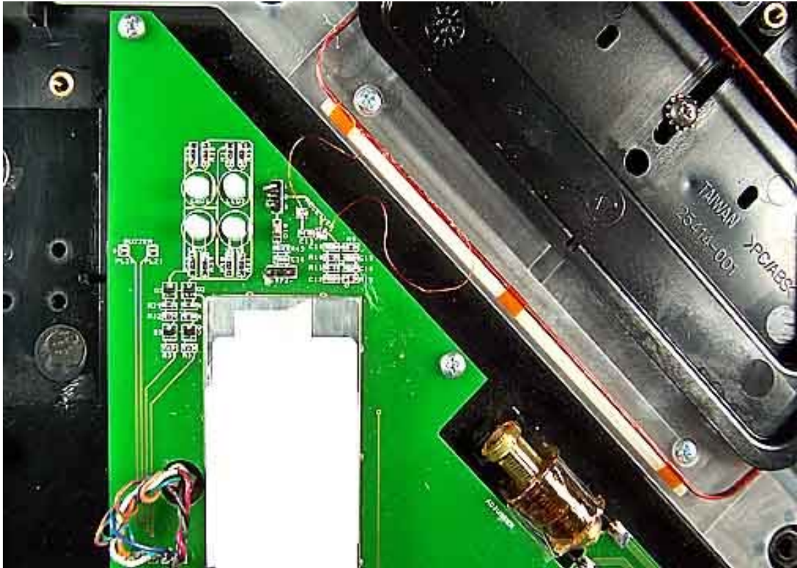
Internal Overview Main PCB Top 2
