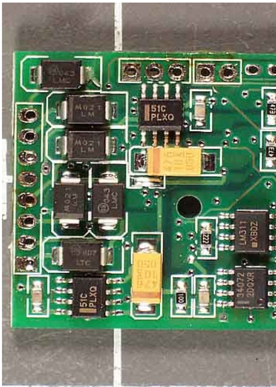
TX PCB Top Closeup 3
