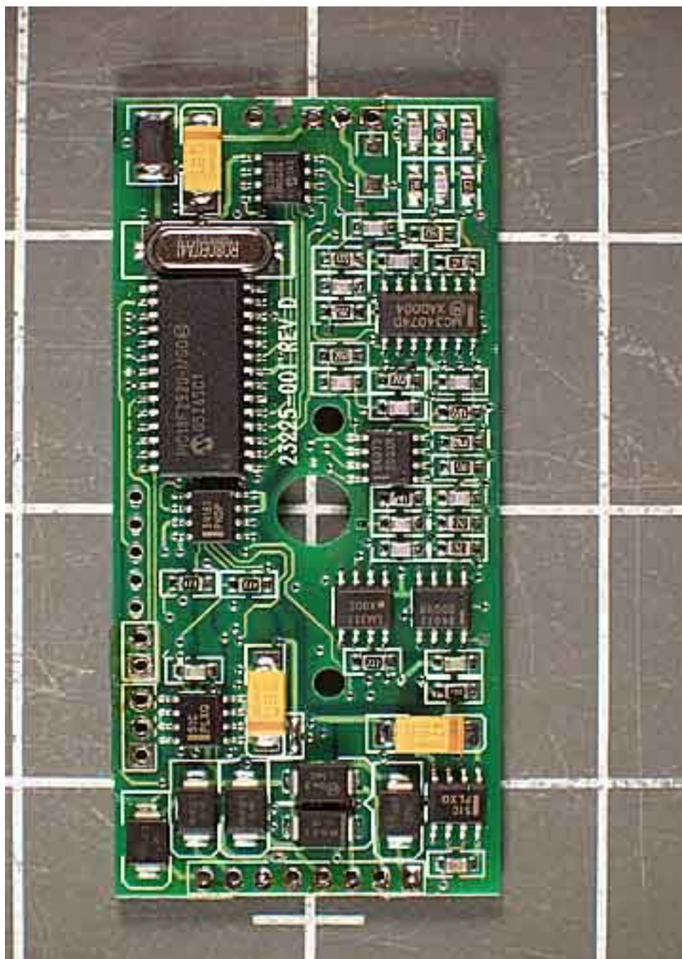
TX PCB Top with Shield Removed
