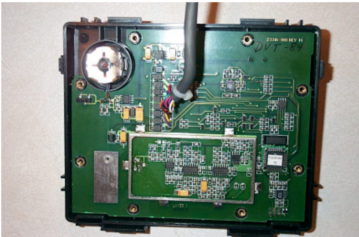
Figure 9.0-2 Transceiver PCB top view with RF shield removed
