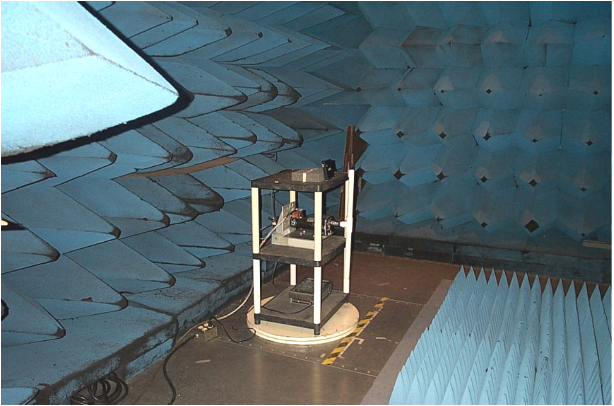
Figure C – 1 Radiated Spurious Emissions Prescan Test Setup, Chamber
