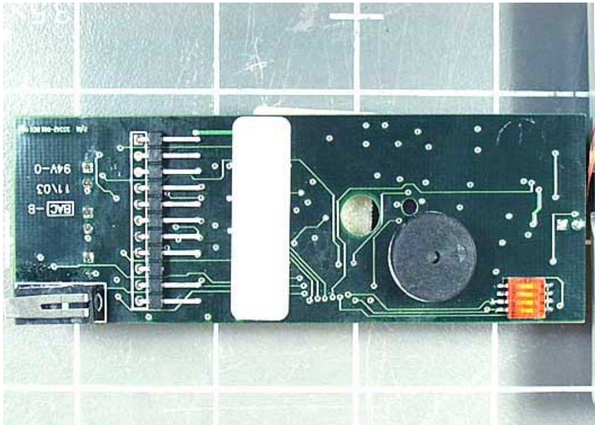
PCB Back
