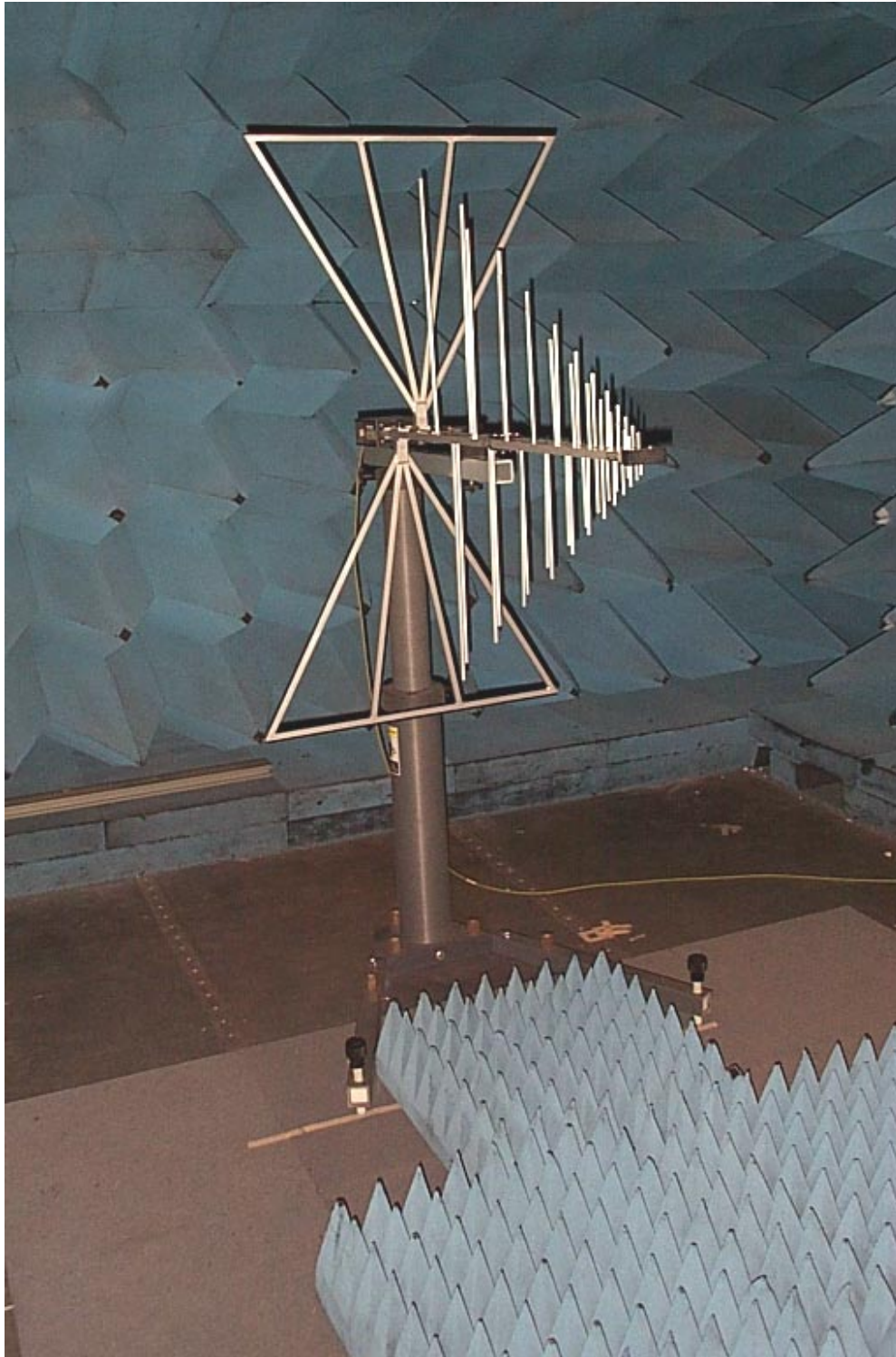
Figure H – 5 Radiated Spurious Emissions Prescan Test Setup, 30MHz - 1GHz
