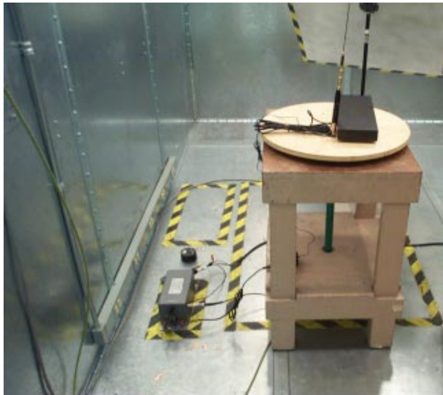
Figure H – 10 Base Station; Conducted Emissions Test Setup
