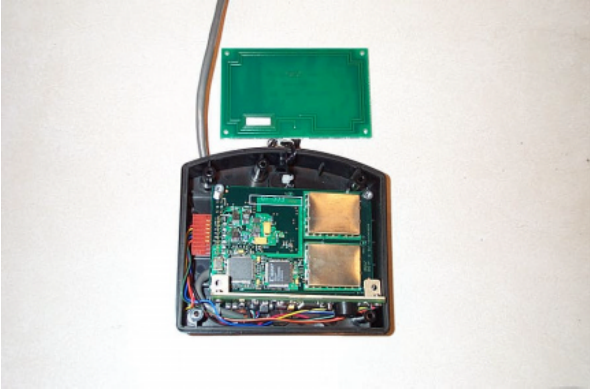
Figure 9.0-2 Top view Serial CAD board (Antenna out)
