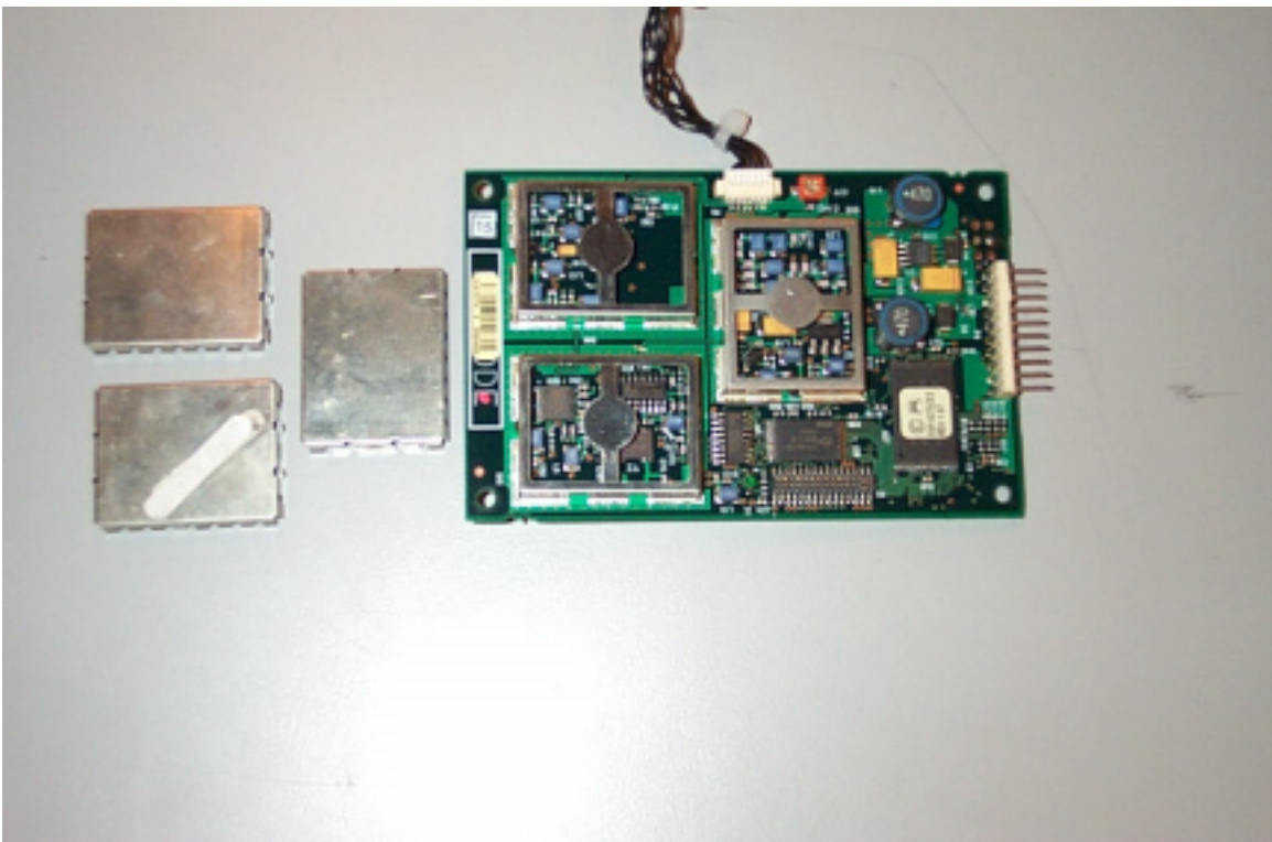
Figure 9.0-5 Bottom view of Serial CAD board w/shields removed
