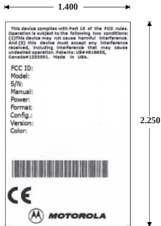
Figure 1.0-1 Maui FCC label Display
