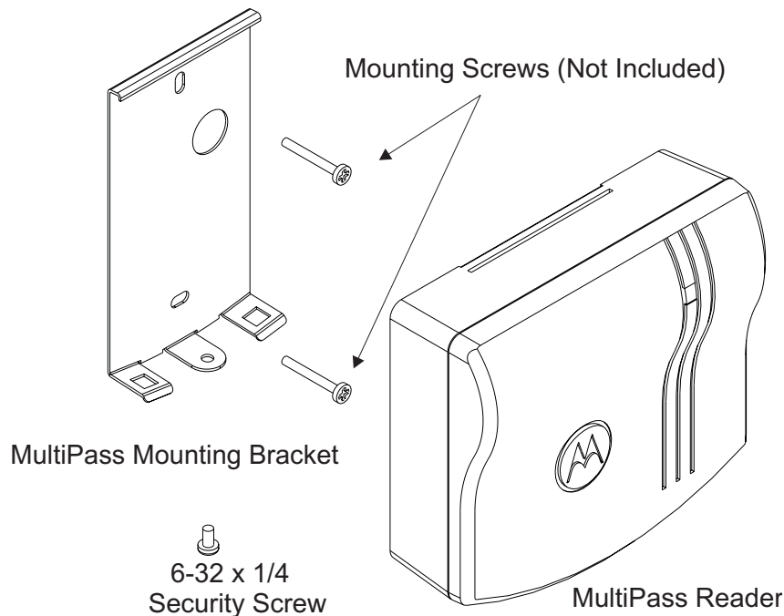
Figure 5 Wall Mounting
