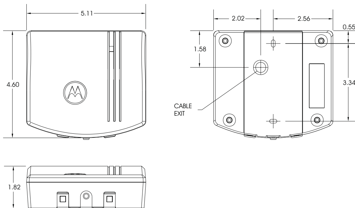
Figure 10 M-Smart™ MultiPass Mechanical Dimensions
