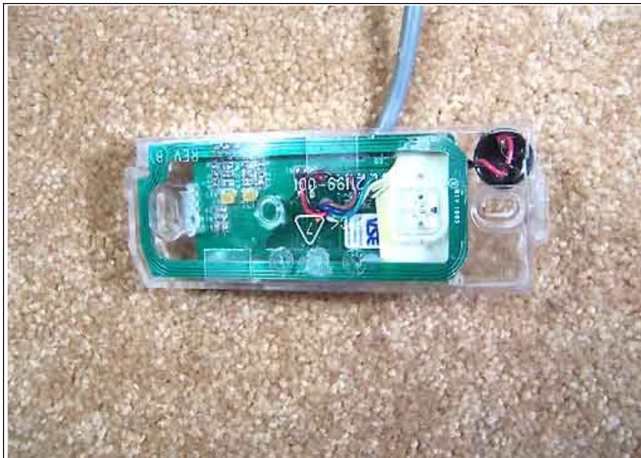
Un-Potted Front
