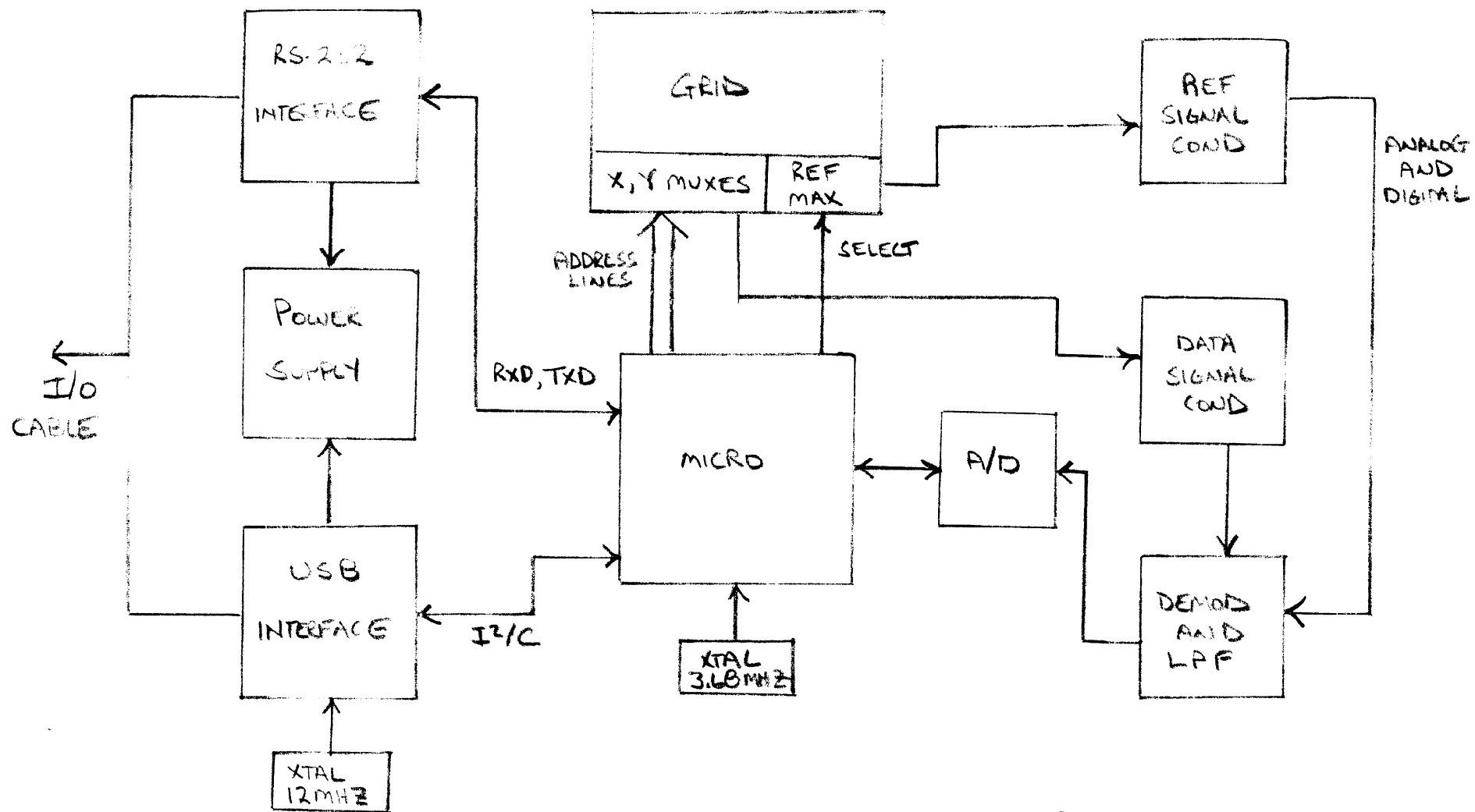
DIGITIZER MODEL 36090 BLOCK DIAGRAM
