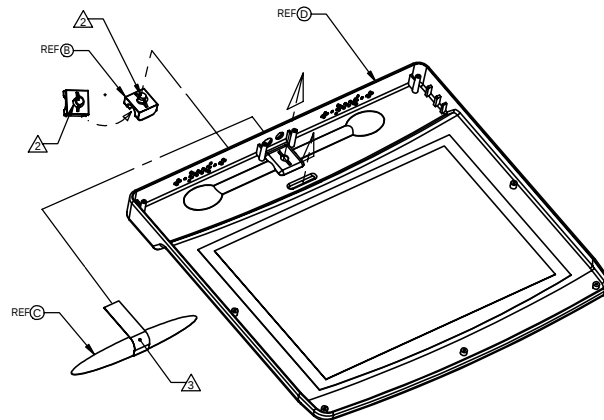
VIEW B - B SCALE: NONE VIEW SHOWN W/O PWB & BASE ATTACHED FOR CLARITY
