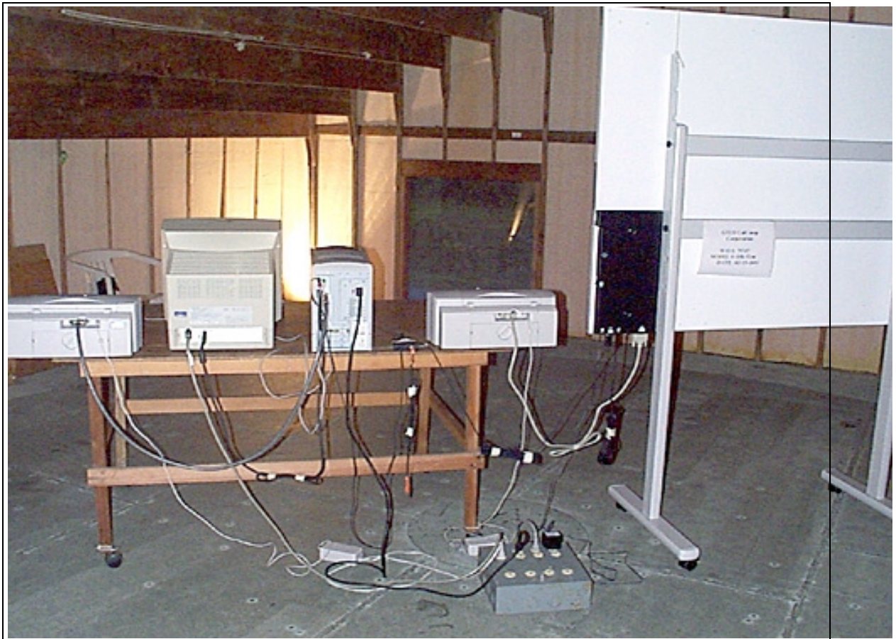
Receiver Radiated Emissions - Back View (Serial)
