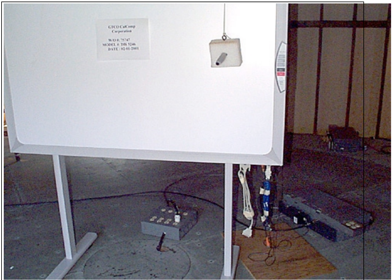
Transmitter Conducted Emissions - Front View
