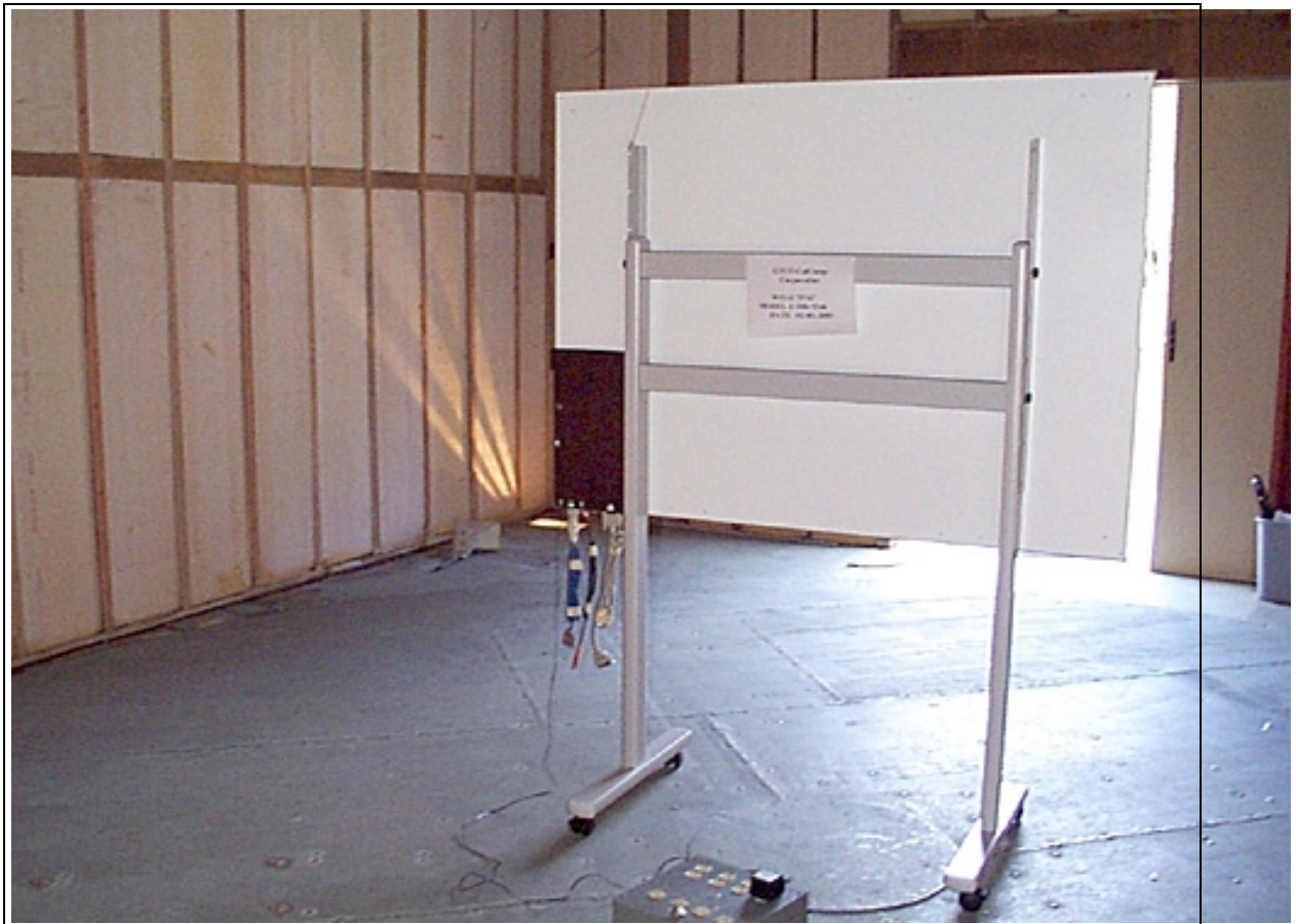
Transmitter Radiated Emissions - Back View
