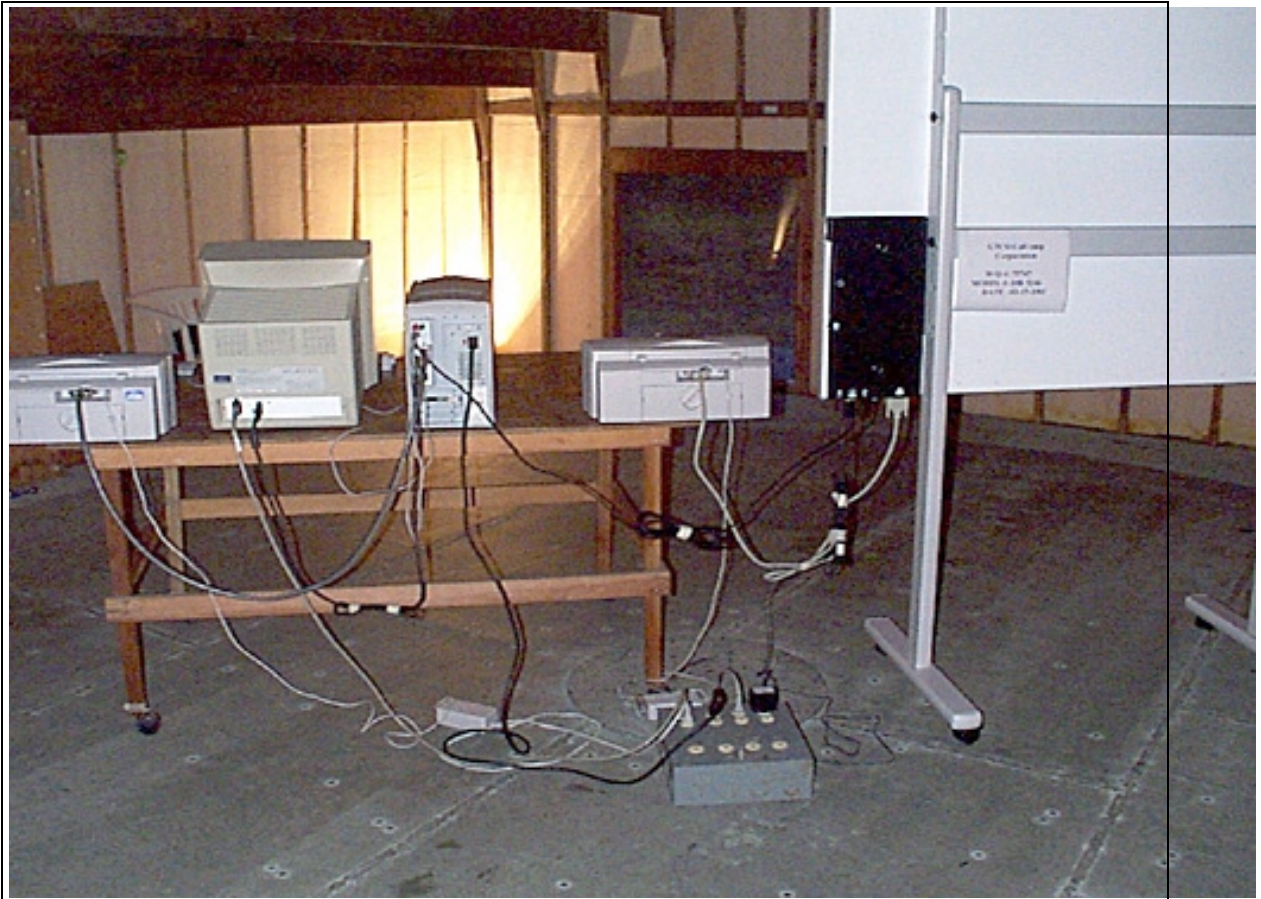
Receiver Radiated Emissions - Back View (USB)
