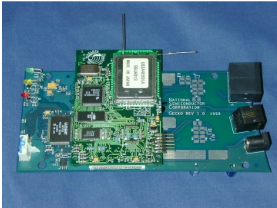
Photo 1 - Base main PCB with RF PCB
