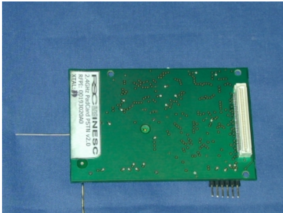
Photo 3 - RF PCB Trace Side
