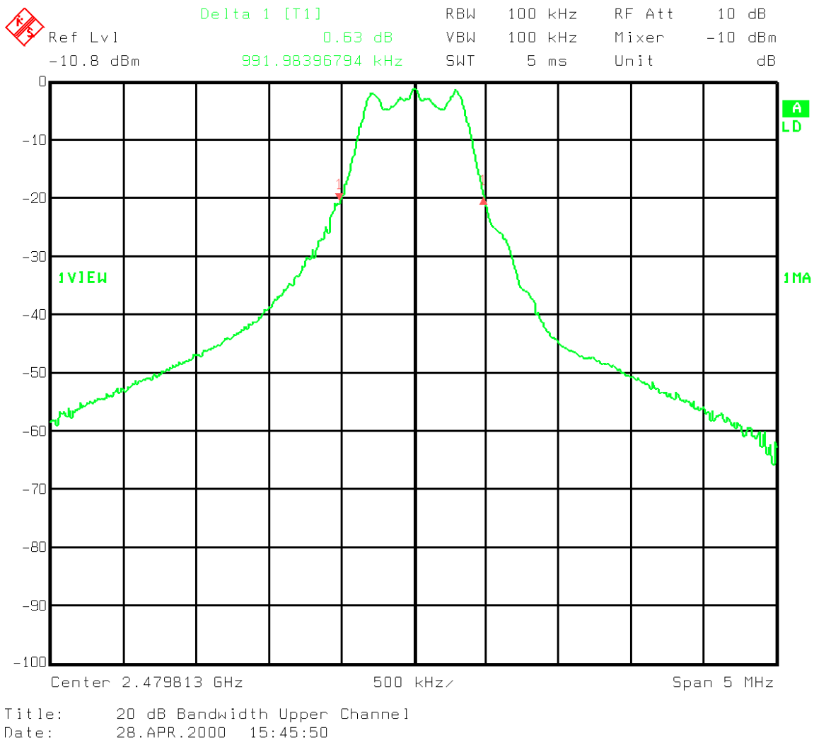
Graph 2 - Occupied Bandwidth upper edge
