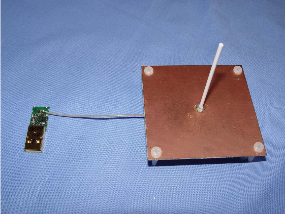
Dongle with external antenna
