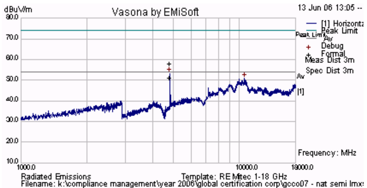
Plot 31 Radiated Emissions for Channel 2402 Antenna #3 - 0.5 dBi Integral Antenna Factor
