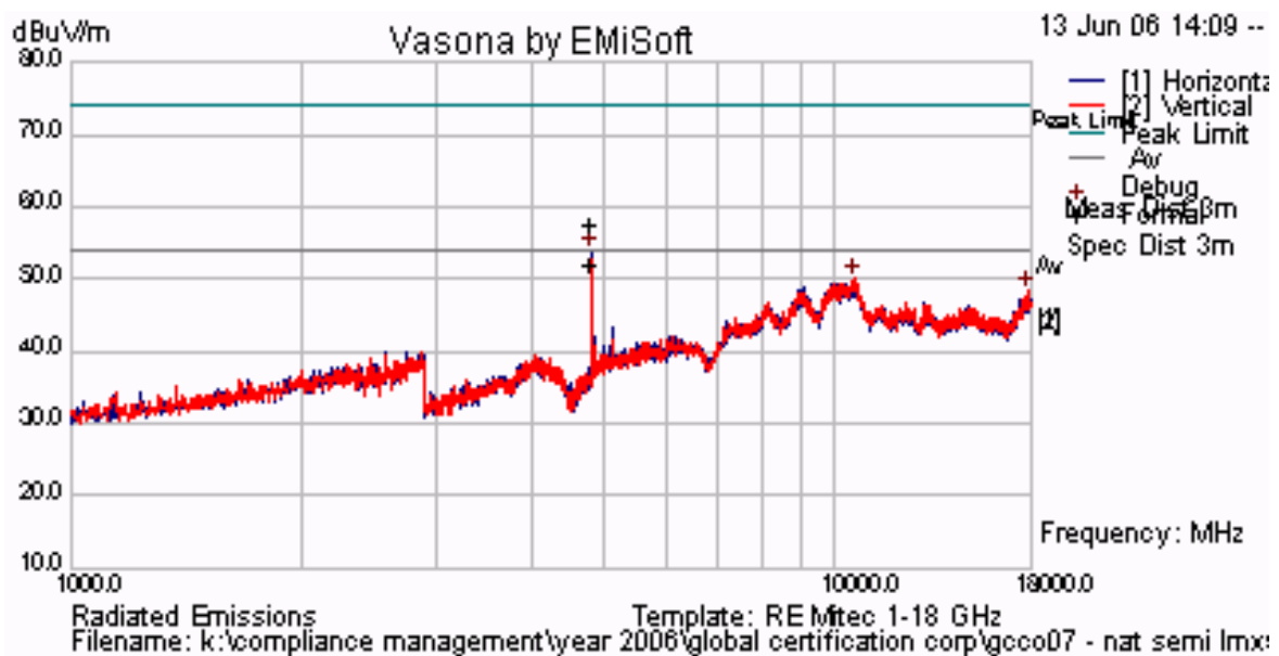
Plot 34 Radiated Emissions for Channel 2402 Antenna #4 - 1 dBi Integral Johanson Tech
