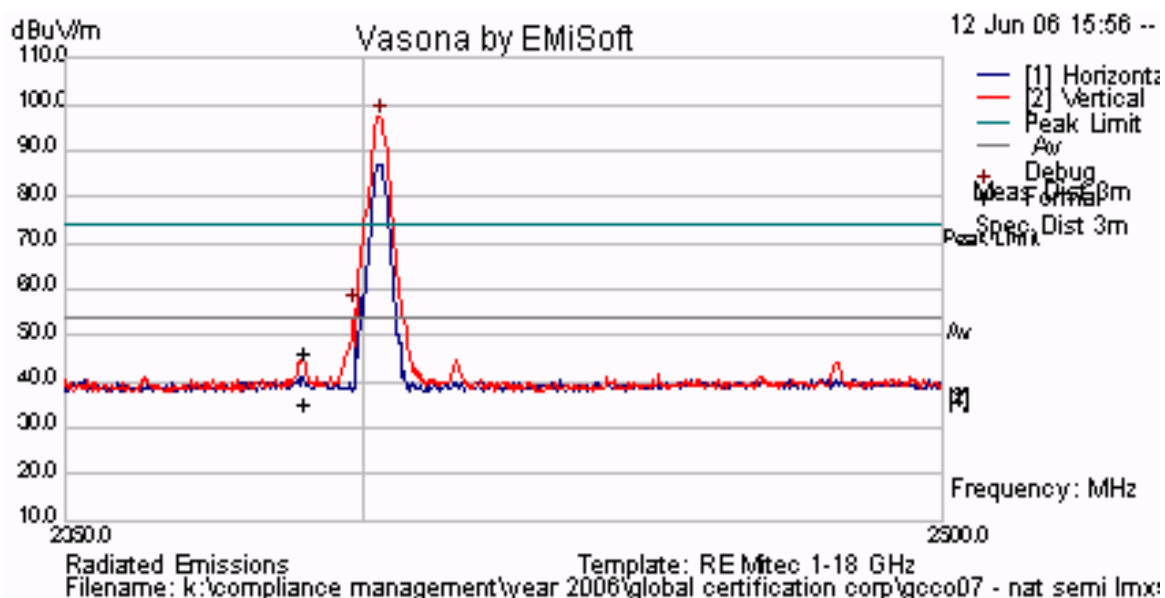
Plot 40 Channel 1 - Lower Band Edge, Peak Emission = 97.04 dBuV/m
