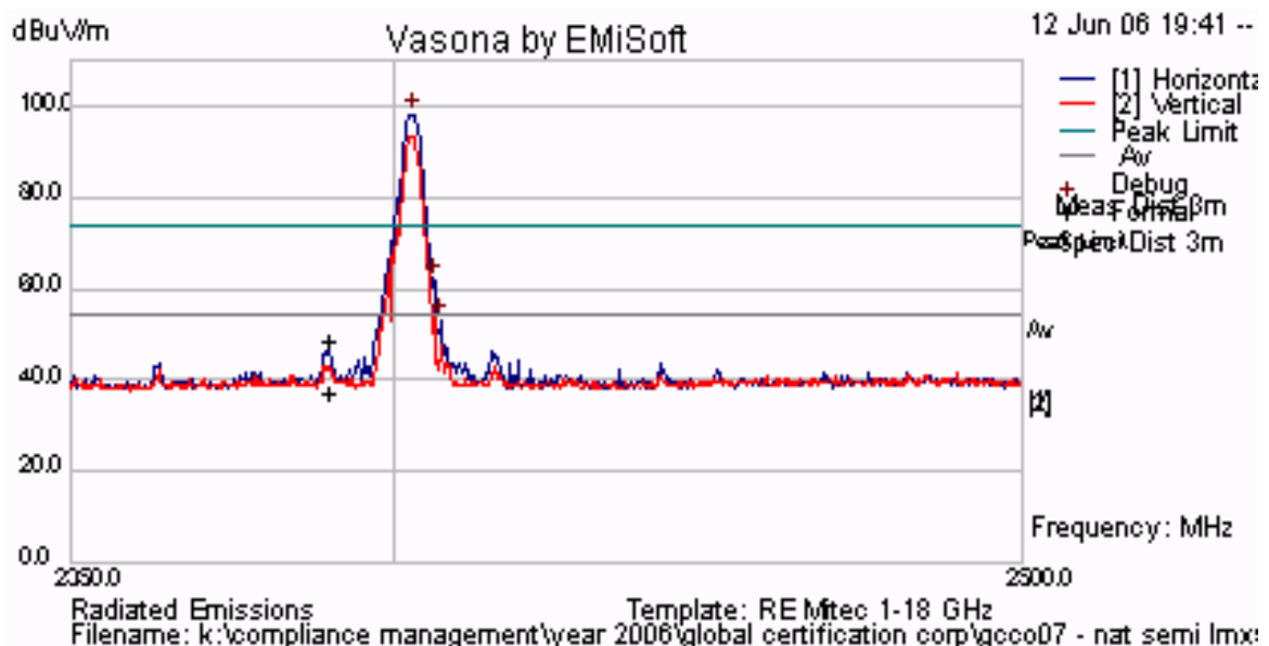
Plot 37 Channel 1 - Lower Band Edge, Peak Emission = 98.2 dBuV/m
