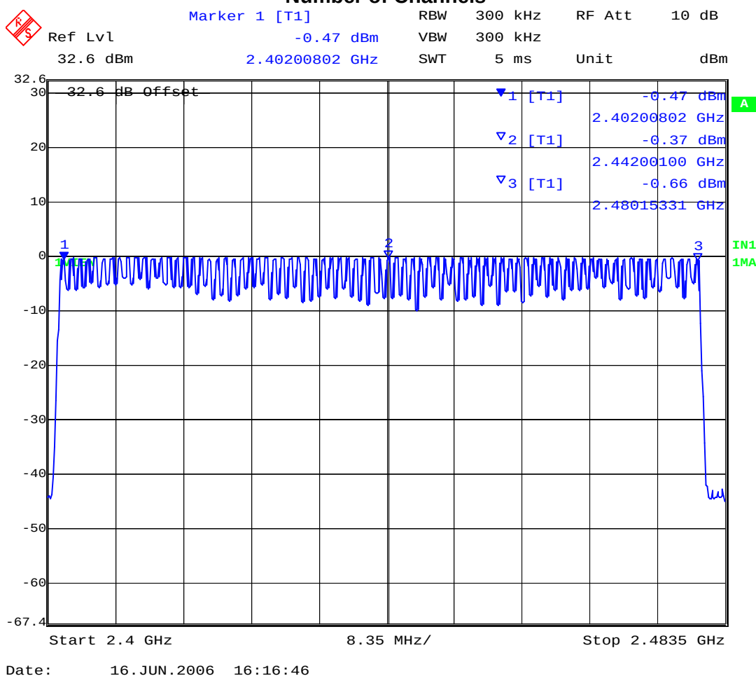
Plot 07 Number of Channels
