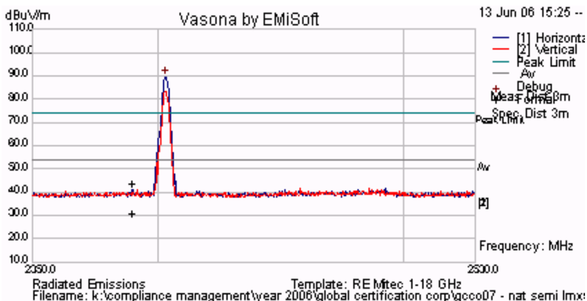
Plot 43 Channel 1 - Lower Band Edge, Peak Emission = 89.54 dBuV/m
