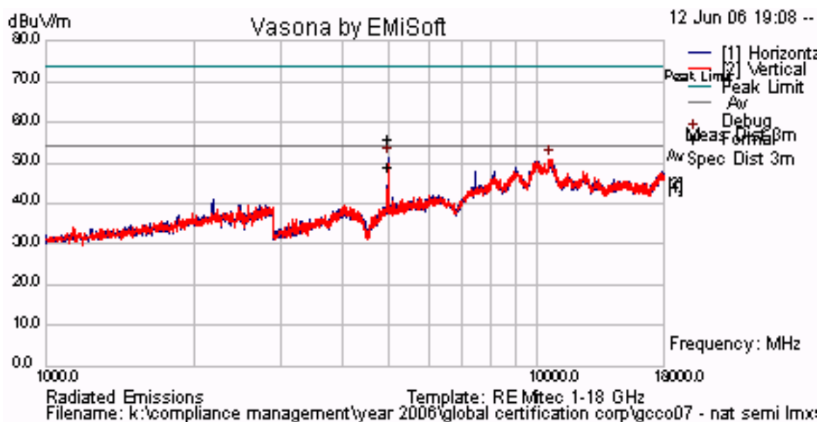
Plot 27 Radiated Emissions for Channel 2480 Antenna #1 - 1 dBi Integral Murata
