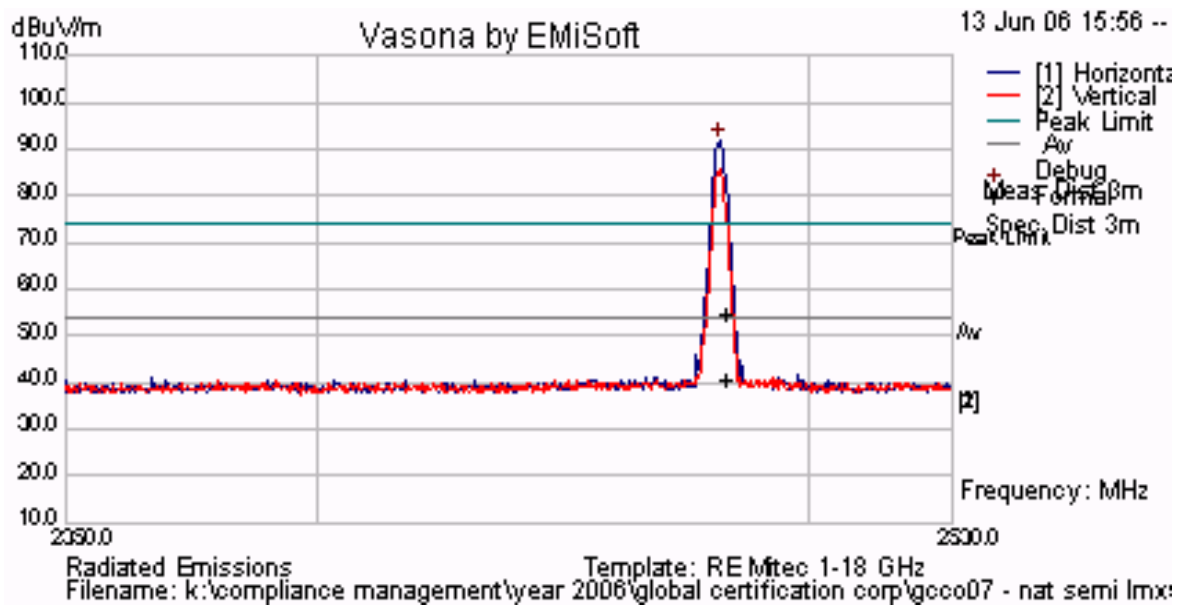
Plot 44 Channel 80 – Upper Band Edge, Peak Emission = 91.68 dB \mu V/m
