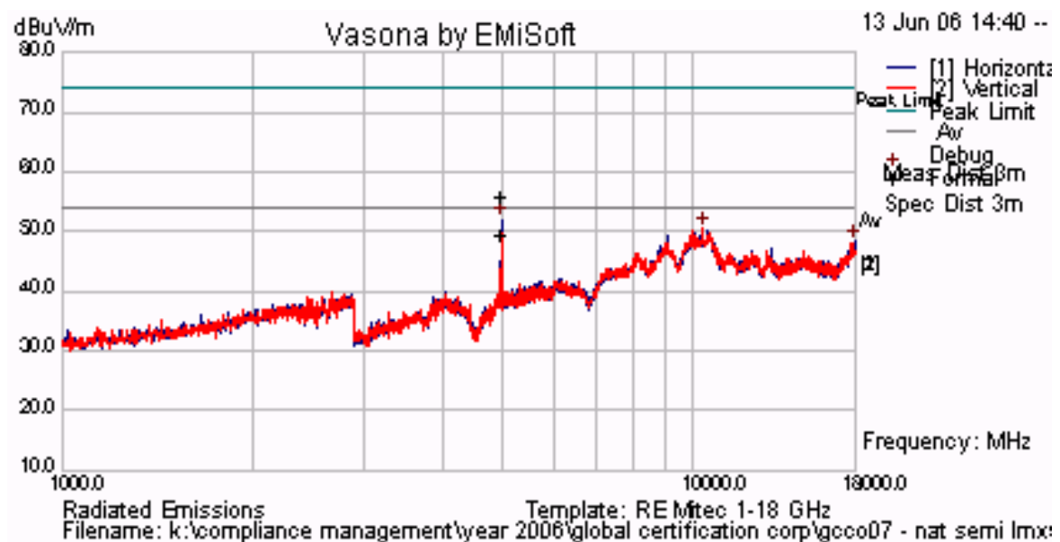
Plot 36 Radiated Emissions for Channel 2480 Antenna #4 - 1 dBi Integral Johanson Tech
