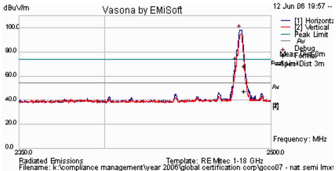
Plot 38 Channel 80 – Upper Band Edge, Peak Emission = 98.34 dB \mu V/m
