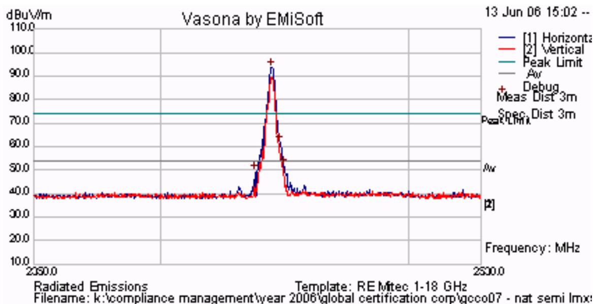
Plot 48 Channel 41 – Peak Field Strength = 93.59 dB \mu V/m
