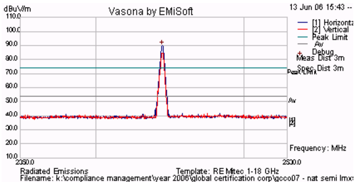
Plot 45 Channel 41 – Peak Field Strength = 89.76 dB \mu V/m
