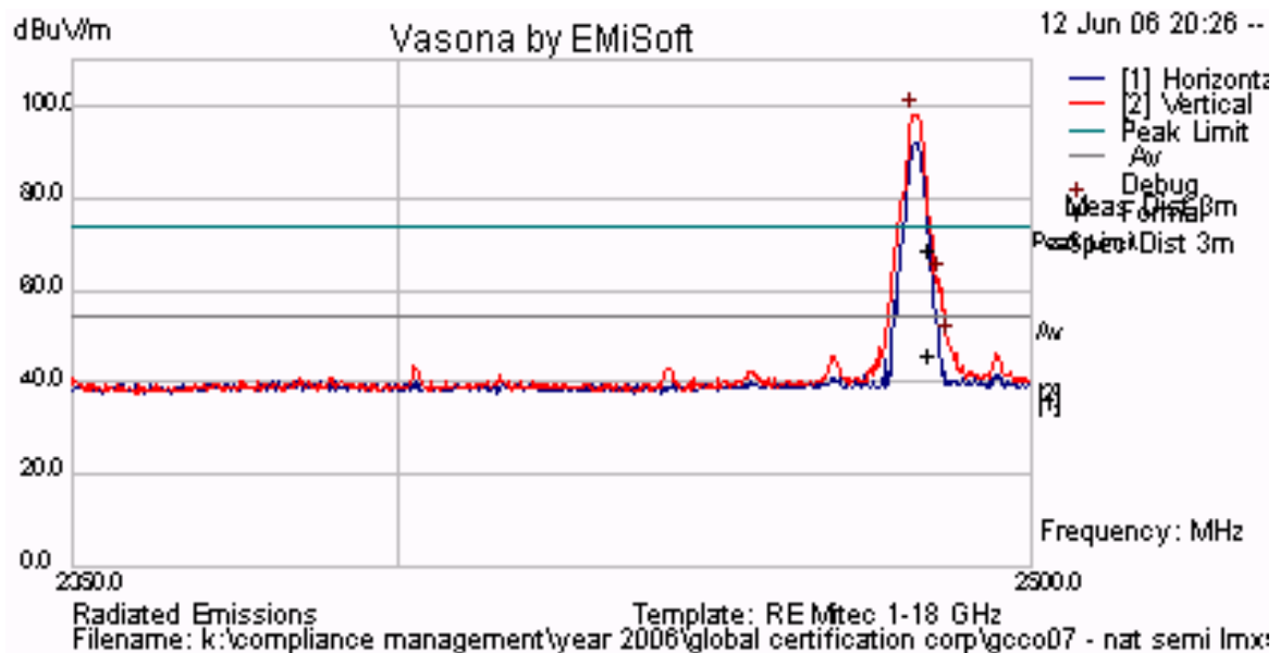
Plot 41 Channel 80 – Upper Band Edge, Peak Emission = 98.34 dB \mu V/m
