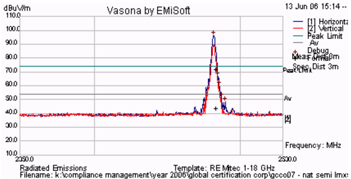
Plot 47 Channel 80 – Upper Band Edge, Peak Emission = 96.02 dB \mu V/m
