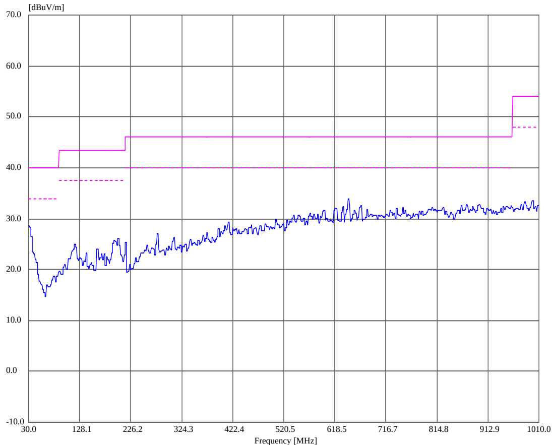
Plot 45 Radiated Emissions 30MHz - 1 GHz
