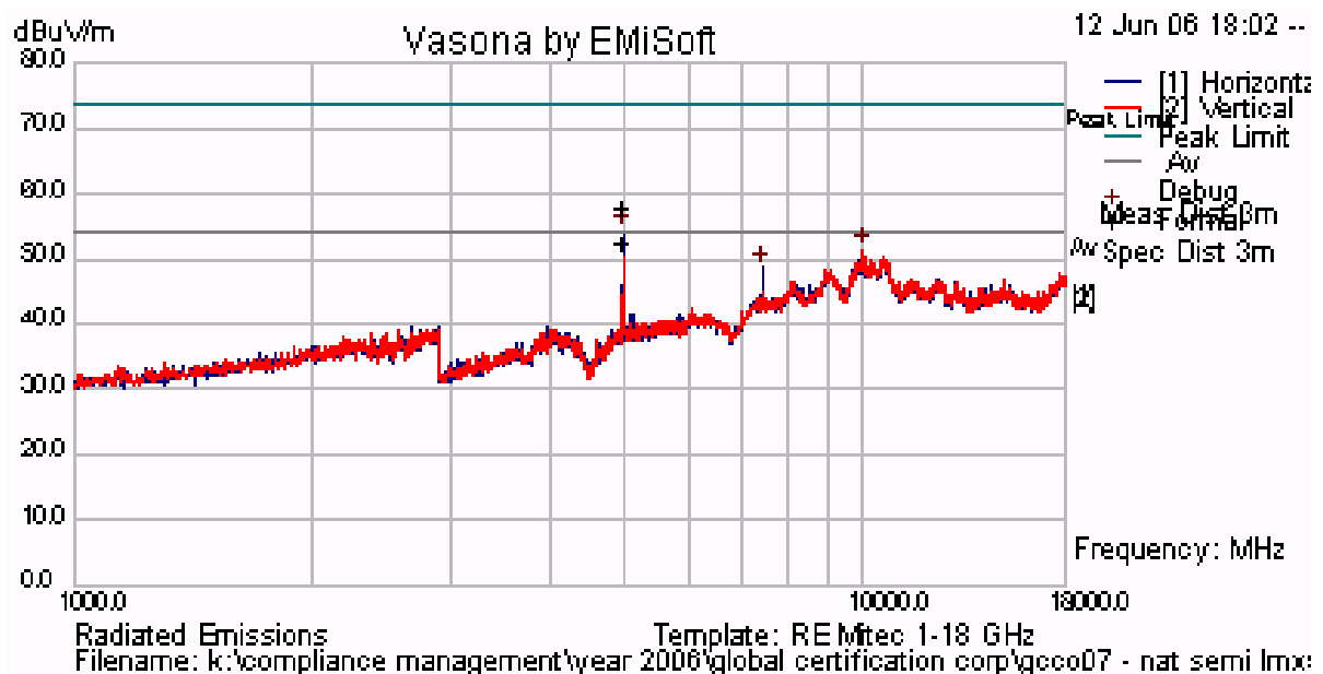
Plot 30 Radiated Emissions for Channel 2480 Antenna #2 - 2 dBi External Wamel Monopole
