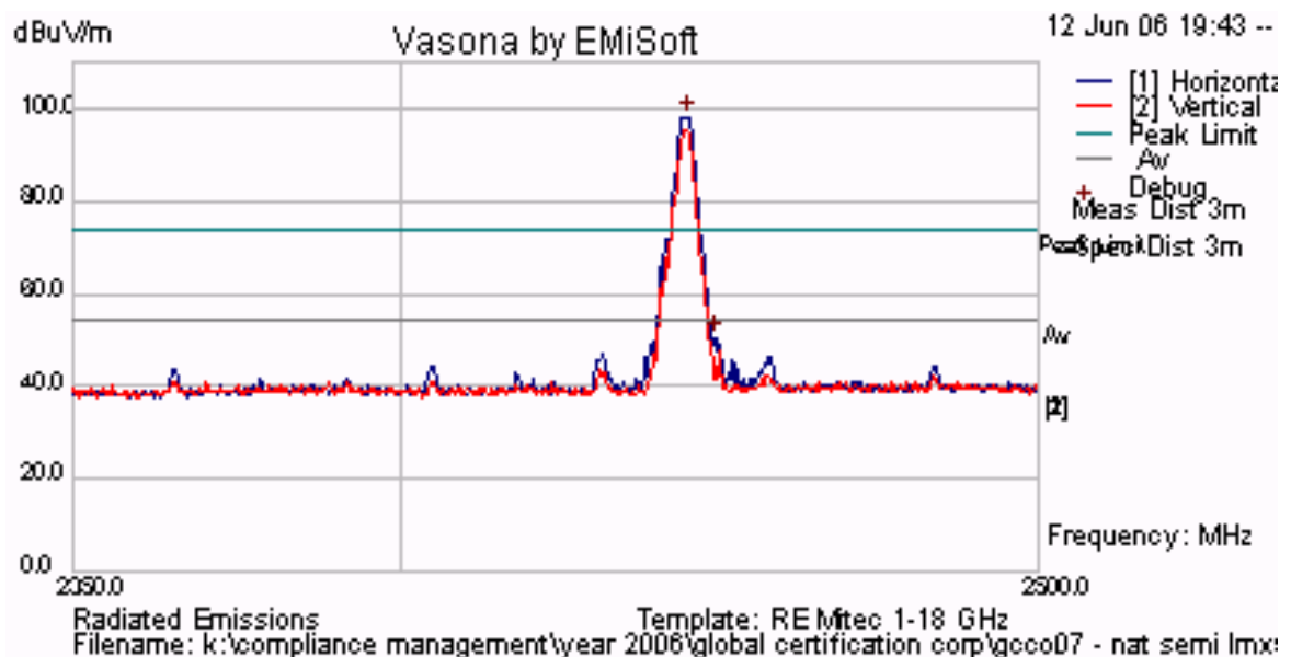
Plot 39 Channel 41 – Peak Field Strength = 98.25 dB \mu V/m
