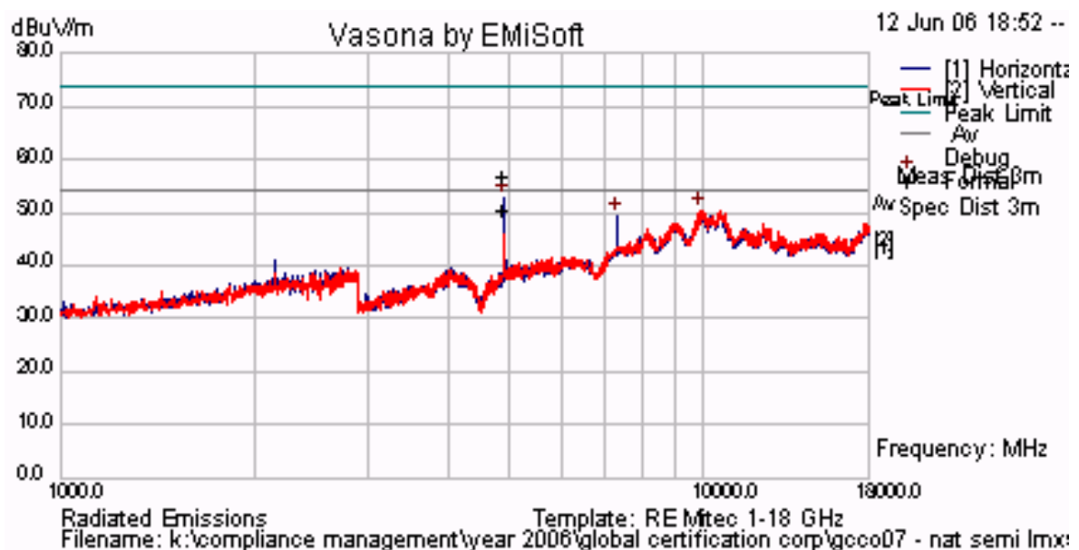
Plot 26 Radiated Emissions for Channel 2441 Antenna #1 - 1 dBi Integral Murata
