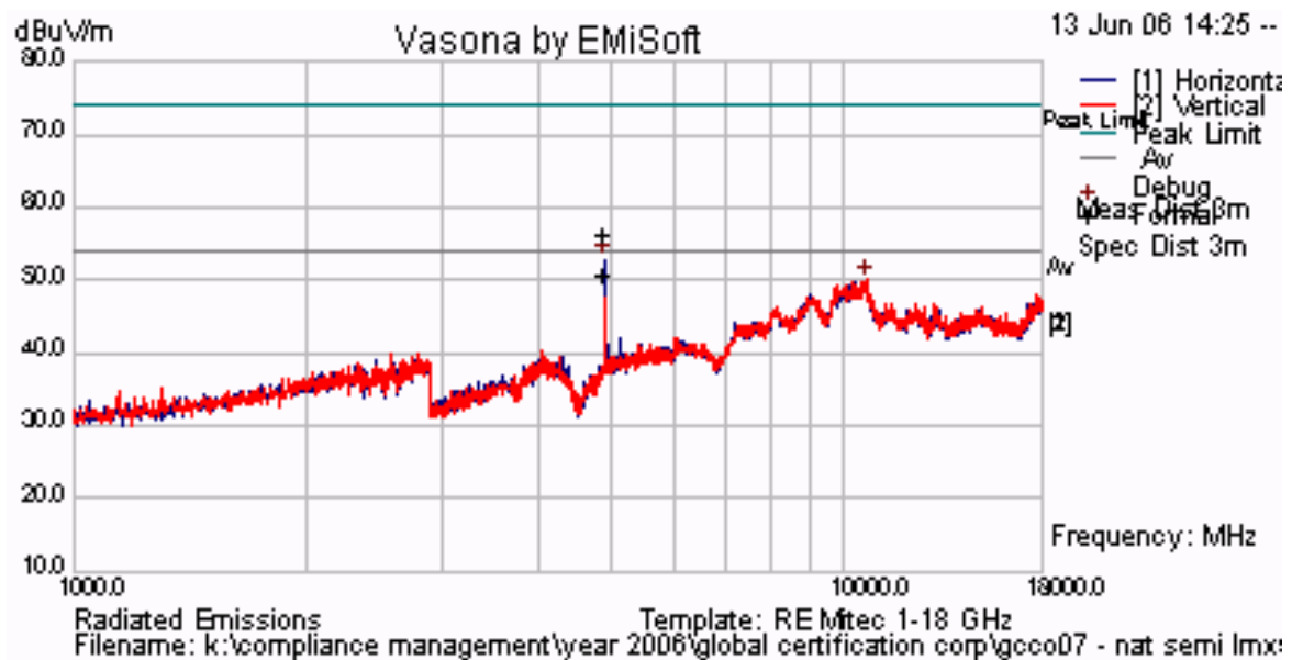
Plot 35 Radiated Emissions for Channel 2441 Antenna #4 - 1 dBi Integral Johanson Tech
