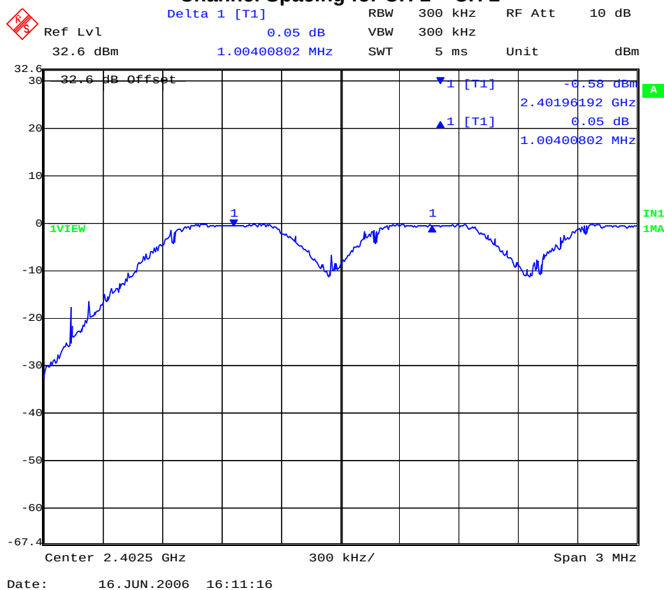
Plot 04 Channel Spacing for CH 1 – CH 2
