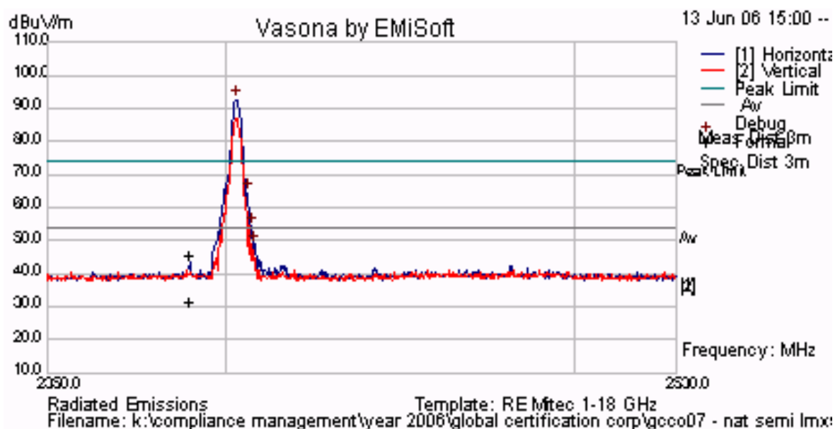
Plot 46 Channel 1 - Lower Band Edge, Peak Emission = 92.71 dBuV/m
