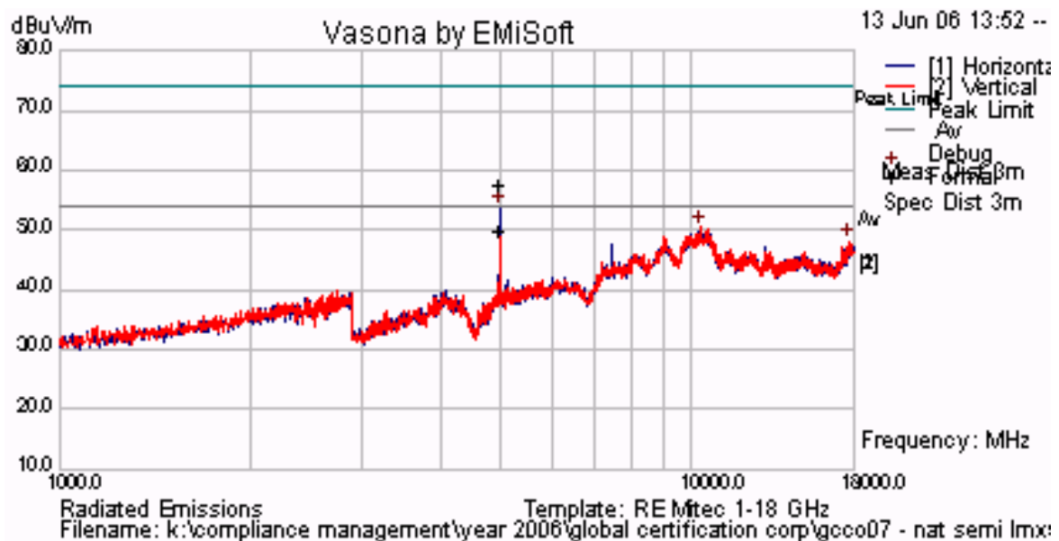
Plot 33 Radiated Emissions for Channel 2480 Antenna #3 - 0.5 dBi Integral Antenna Factor
