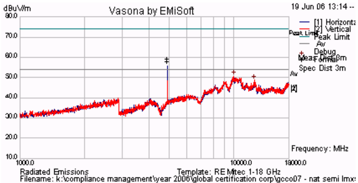
Plot 44 Receiver Radiated Emissions for Ch 41
