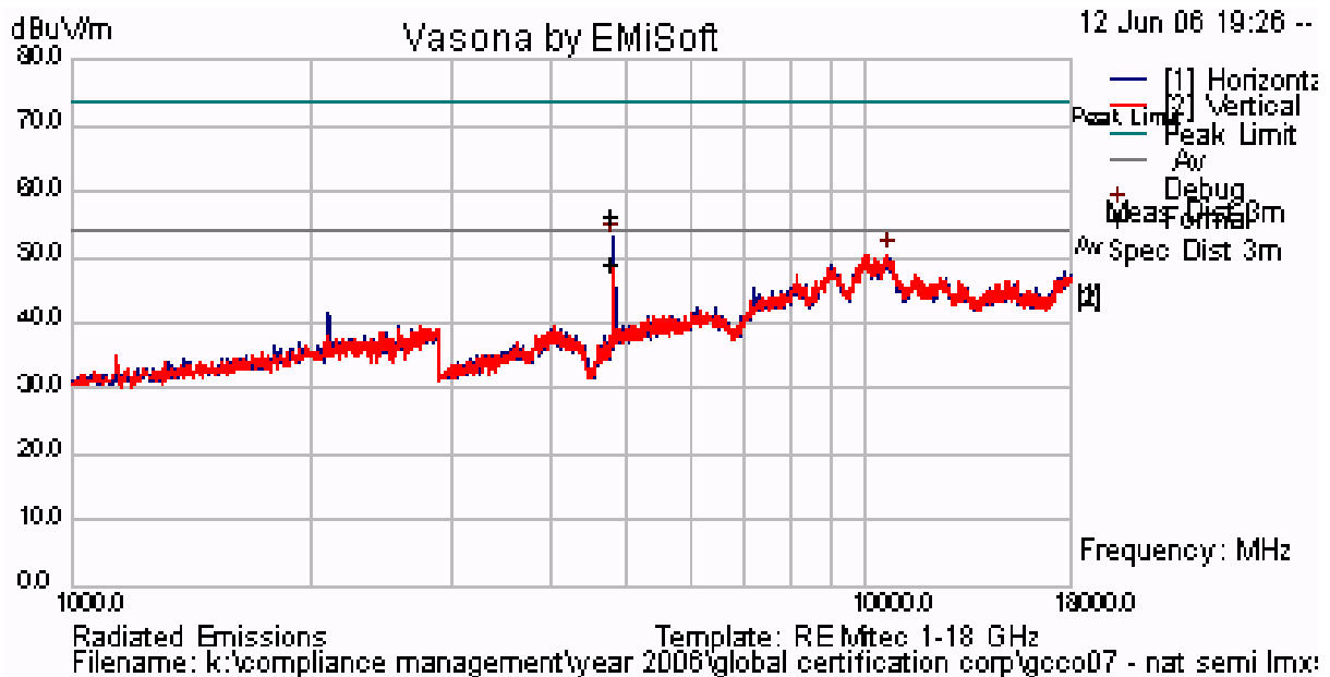
Plot 25 Radiated Emissions for Channel 2402 Antenna #1 - 1 dBi Integral Murata
