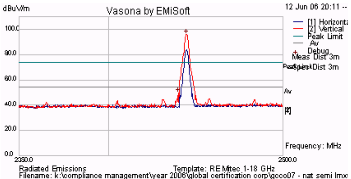
Plot 42 Channel 41 – Peak Field Strength = 96.09 dB \mu V/m
