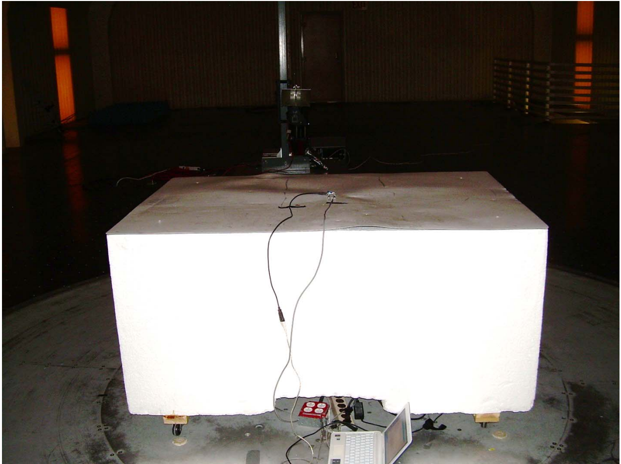
Back View of the Test Setup
