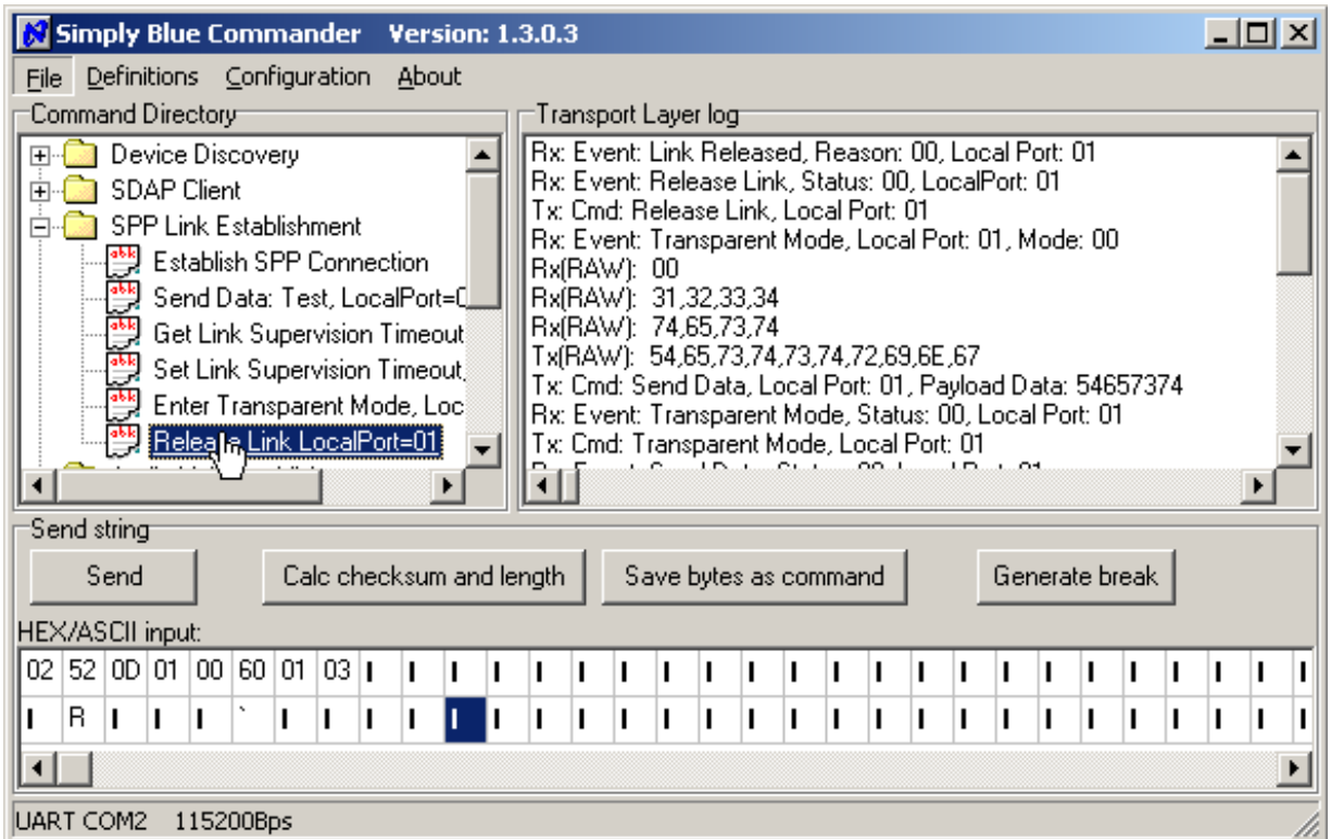
Figure 2-47. Releasing the link by the LMX9830/LMX9838
