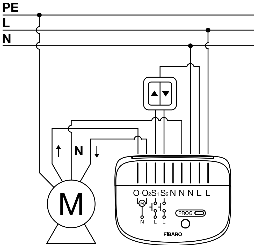
Wiring diagram – connection with AC motor
