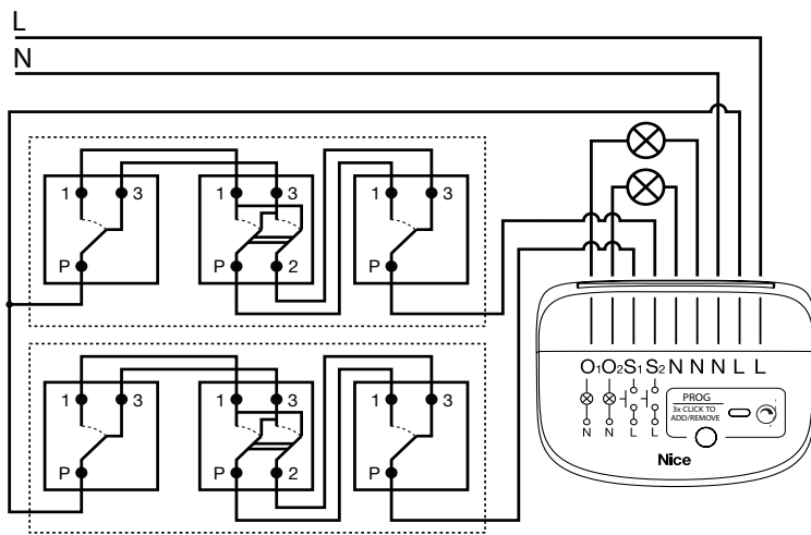
Diagram 8: Stair-cross switches x 2 - - independent outputs
