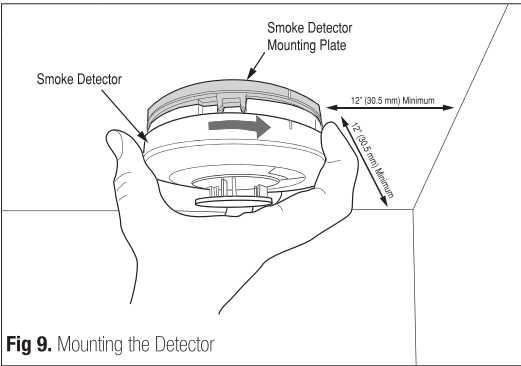
Fig 9. Mounting the Detector
