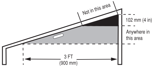
Fig 7. Example of proper mounting for Detectors with sloped ceilings
