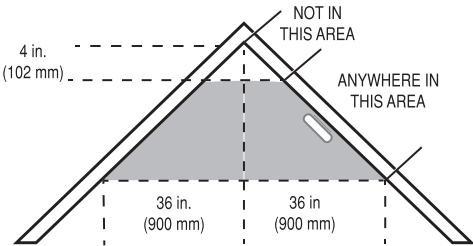
Fig 8. Example of proper mounting for Detectors with peaked ceilings
