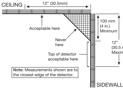
Fig 6. Example of proper mounting for Detectors
