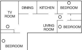
Fig 3. Location of the Detectors in dwelling units with more than one bedroom area or with bedrooms on more than one floor.
