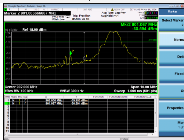
Sub-G LOW CHANNEL, BAND EDGE
