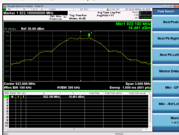
Sub-G HIGH CHANNEL, CARRIER LEVEL
