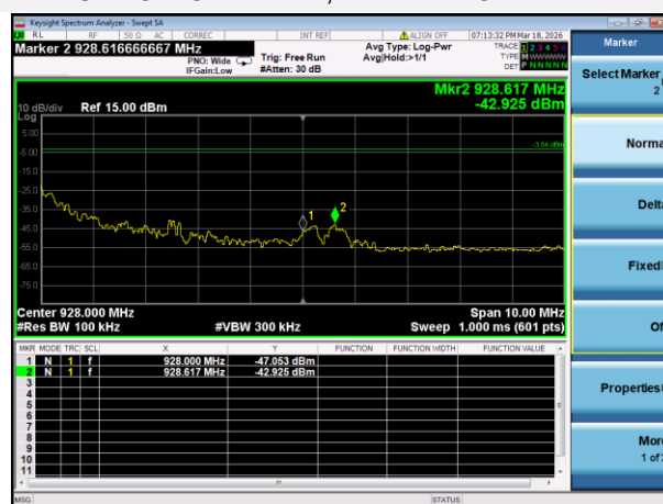
Sub-G HIGH CHANNEL, BAND EDGE
