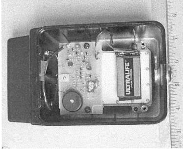
PCB VIEW
