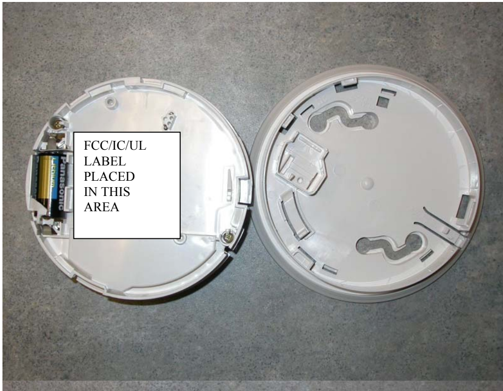
REAR VIEW, DXS-73 SMOKE ALARM FCC / IC LABEL PLACED APPROX. AS SHOWN
