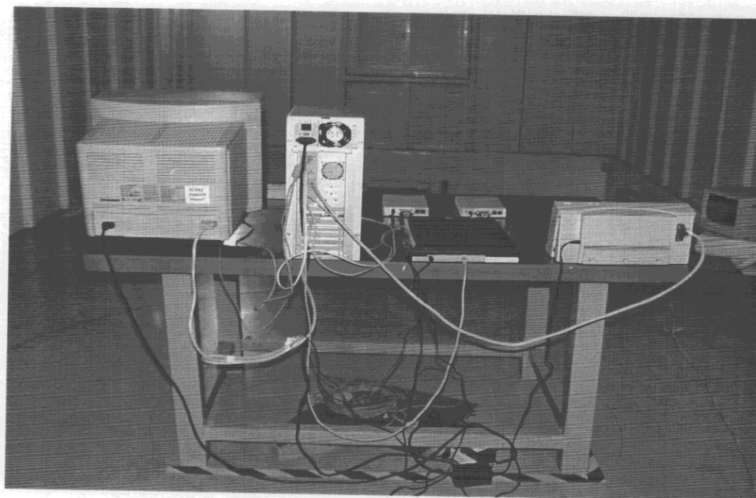
BACK VIEW OF RADIATED TEST ( Mode 1 )
