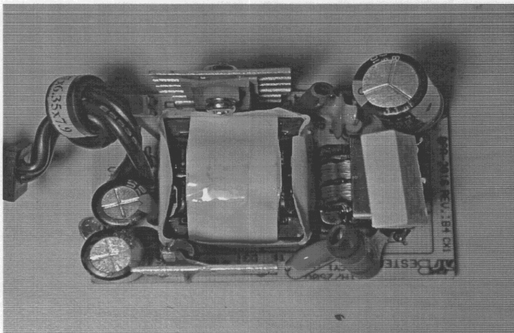
Inner View of Adapter(Mode 3)
