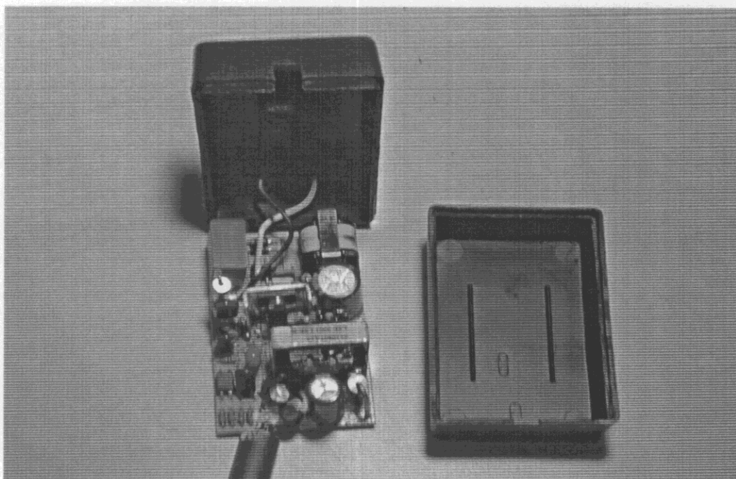
Inner View of Adapter(Mode 1)
