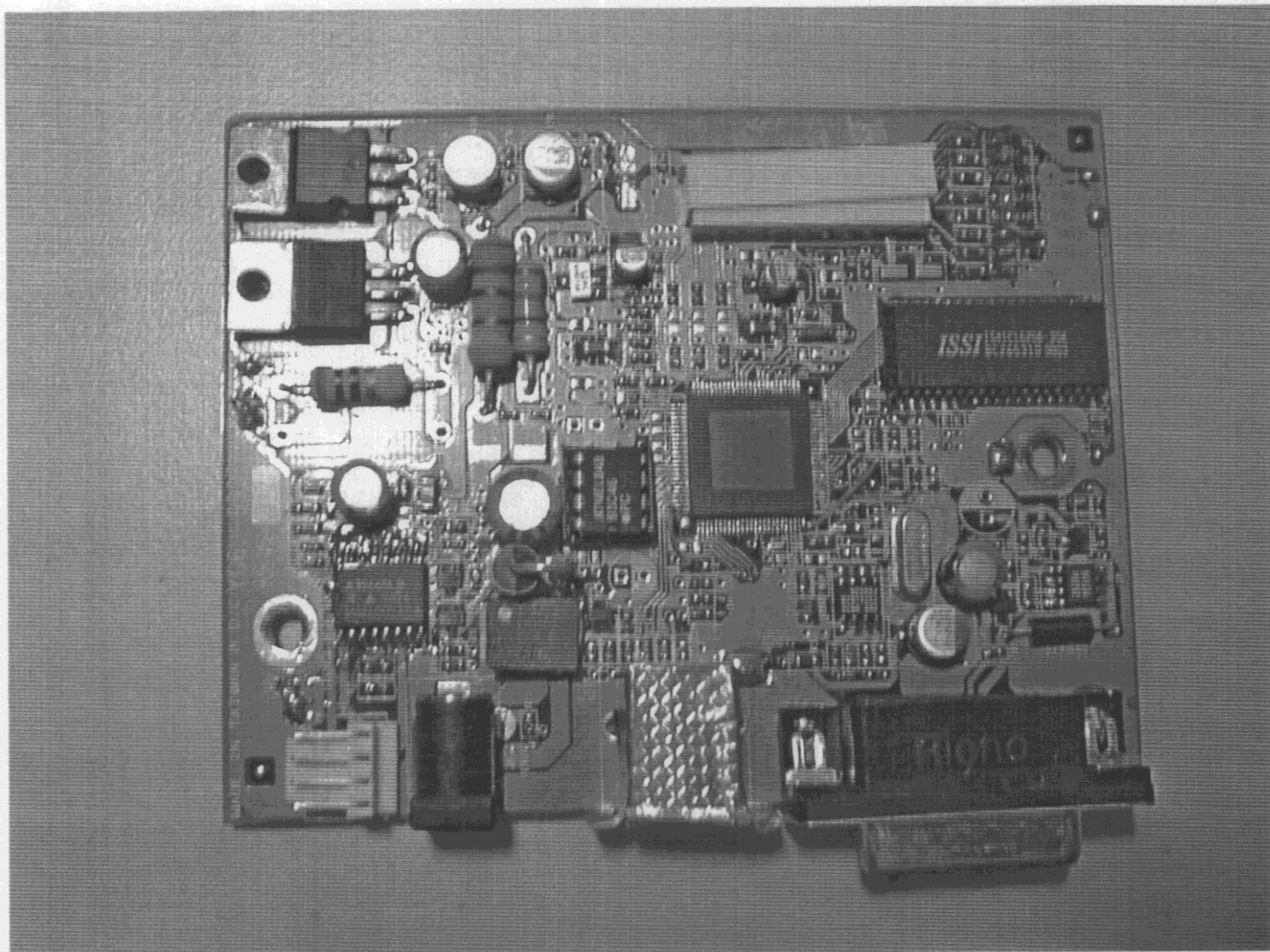
Component Side of Control Board
