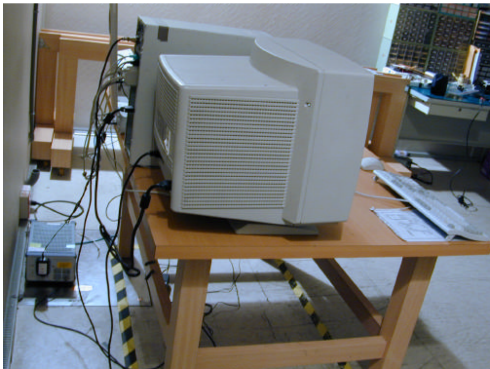
Back View of Conducted Test (Mode 3)
