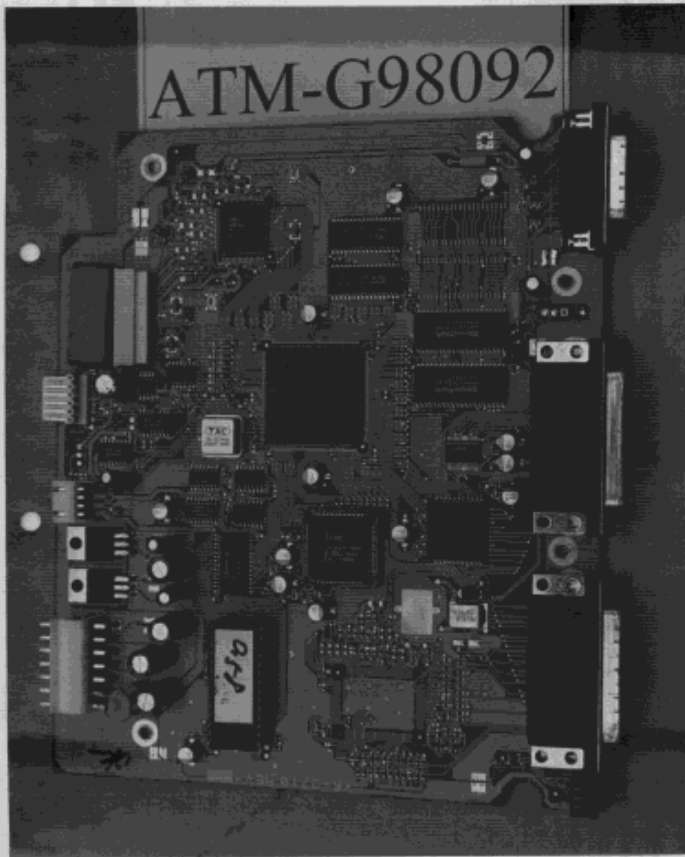
Figure 6 Main Board (Component Side)
