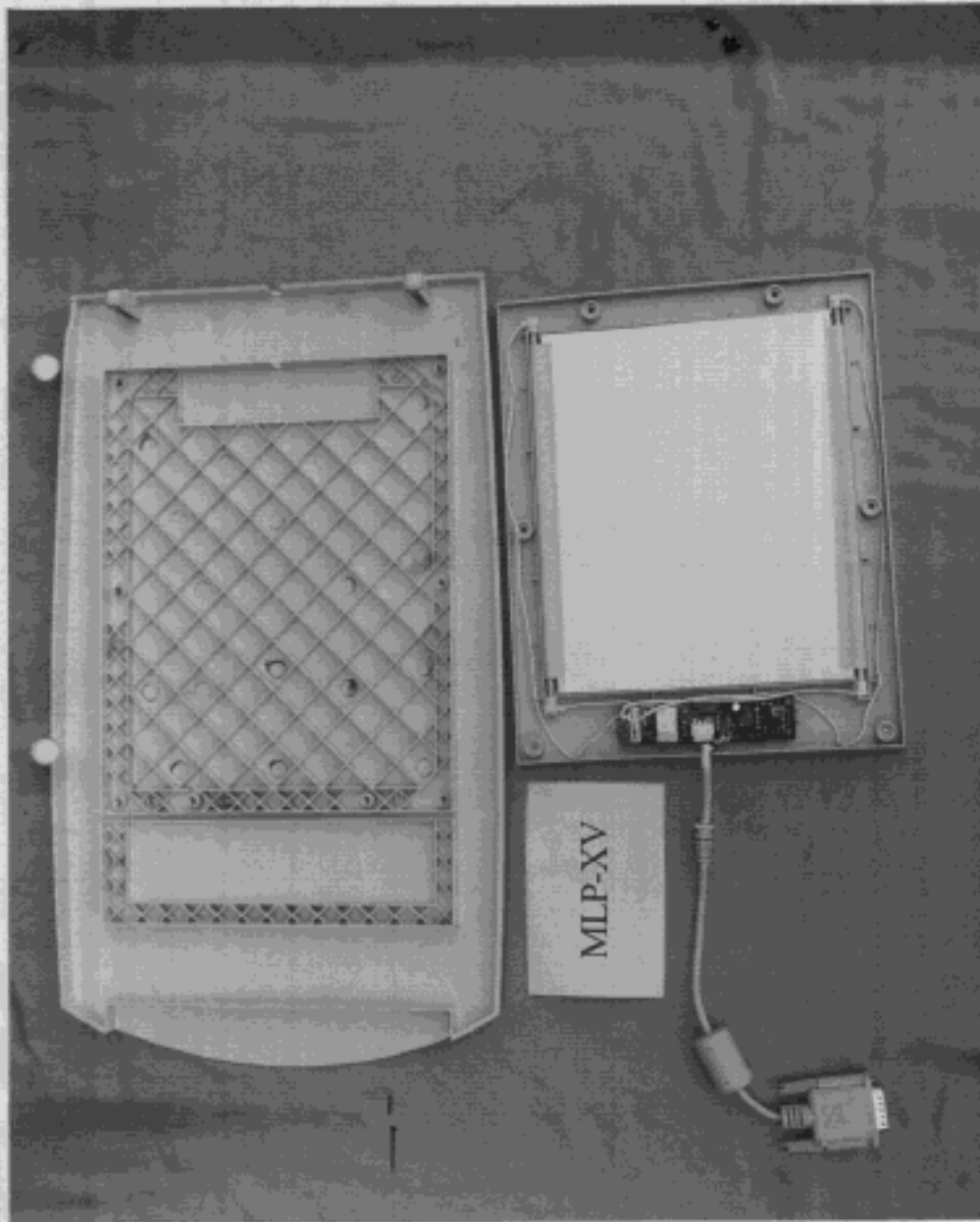
Figure 16 Cover Removed, Internal View of Light Plate
